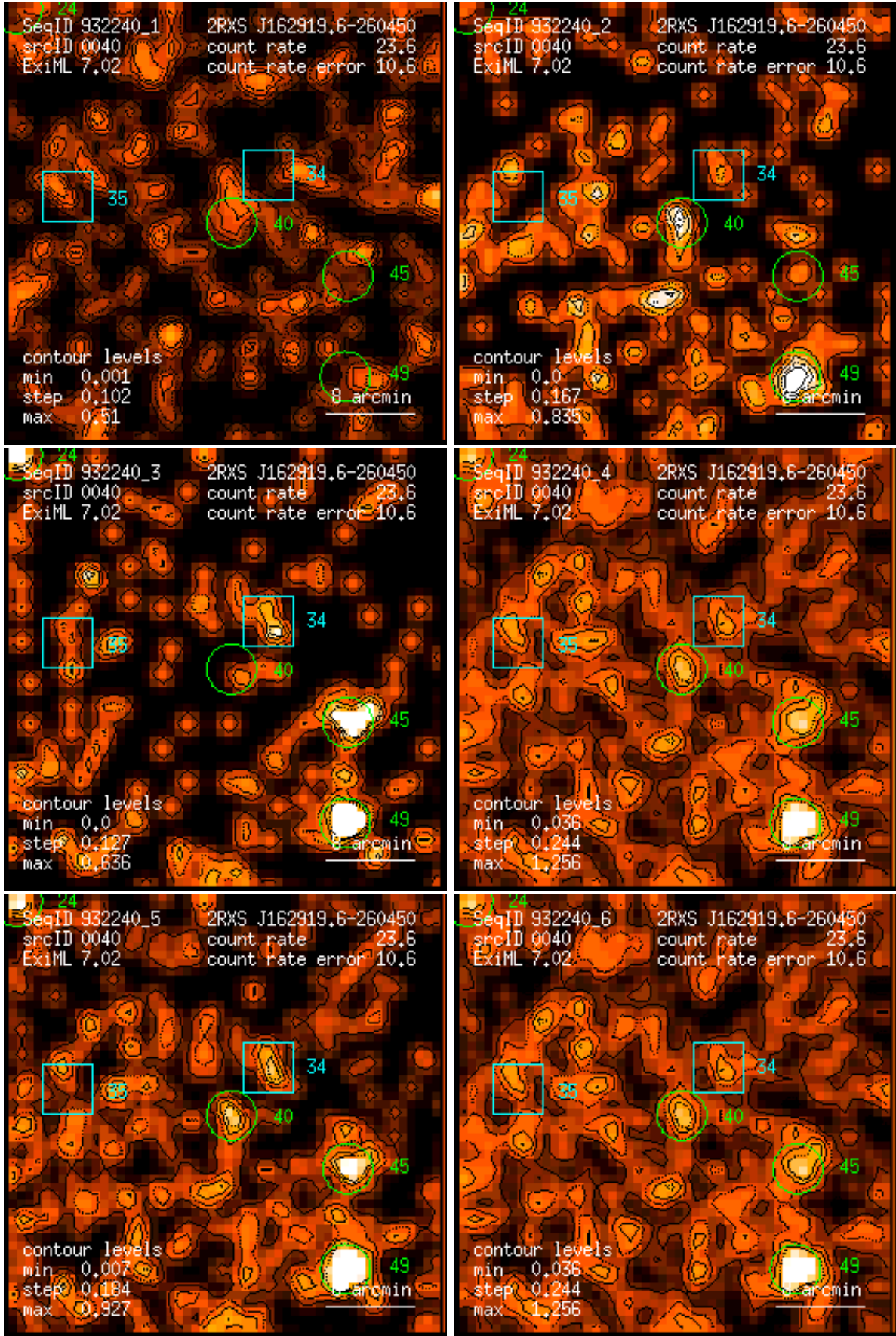
Figure 40: RASS 932240: detection 0040: band rate images, Gaussian filter: (1) PSPC channels 11 – 41, (2) 52 – 90, (3) 91 – 201, (4) 11 – 235, (5) 52 – 201, (6) 11 – 201. Broad band rates in counts/ks. Band rate contour levels in counts/ks/arcmin 2 .
