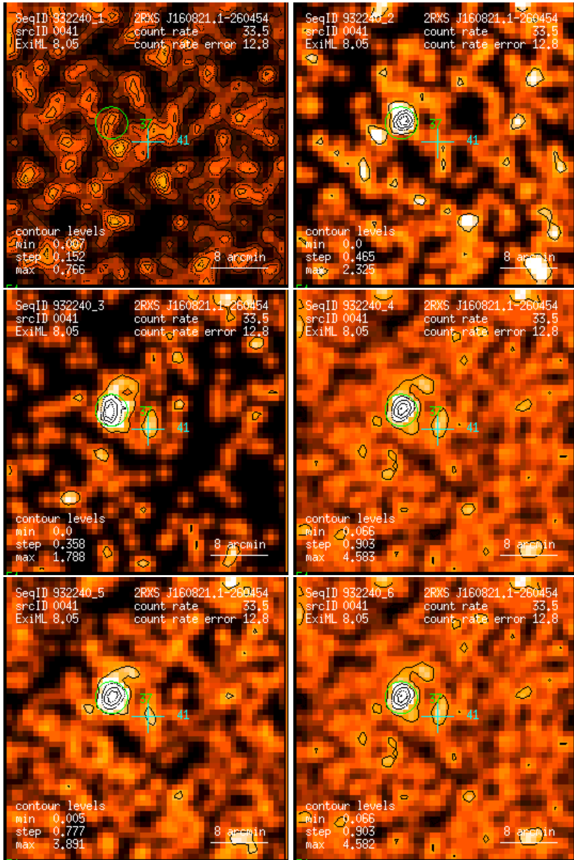
Figure 41: RASS 932240: detection 0041: band rate images, Gaussian filter: (1) PSPC channels 11 – 41, (2) 52 – 90, (3) 91 – 201, (4) 11 – 235, (5) 52 – 201, (6) 11 – 201. Broad band rates in counts/ks. Band rate contour levels in counts/ks/arcmin 2 .
