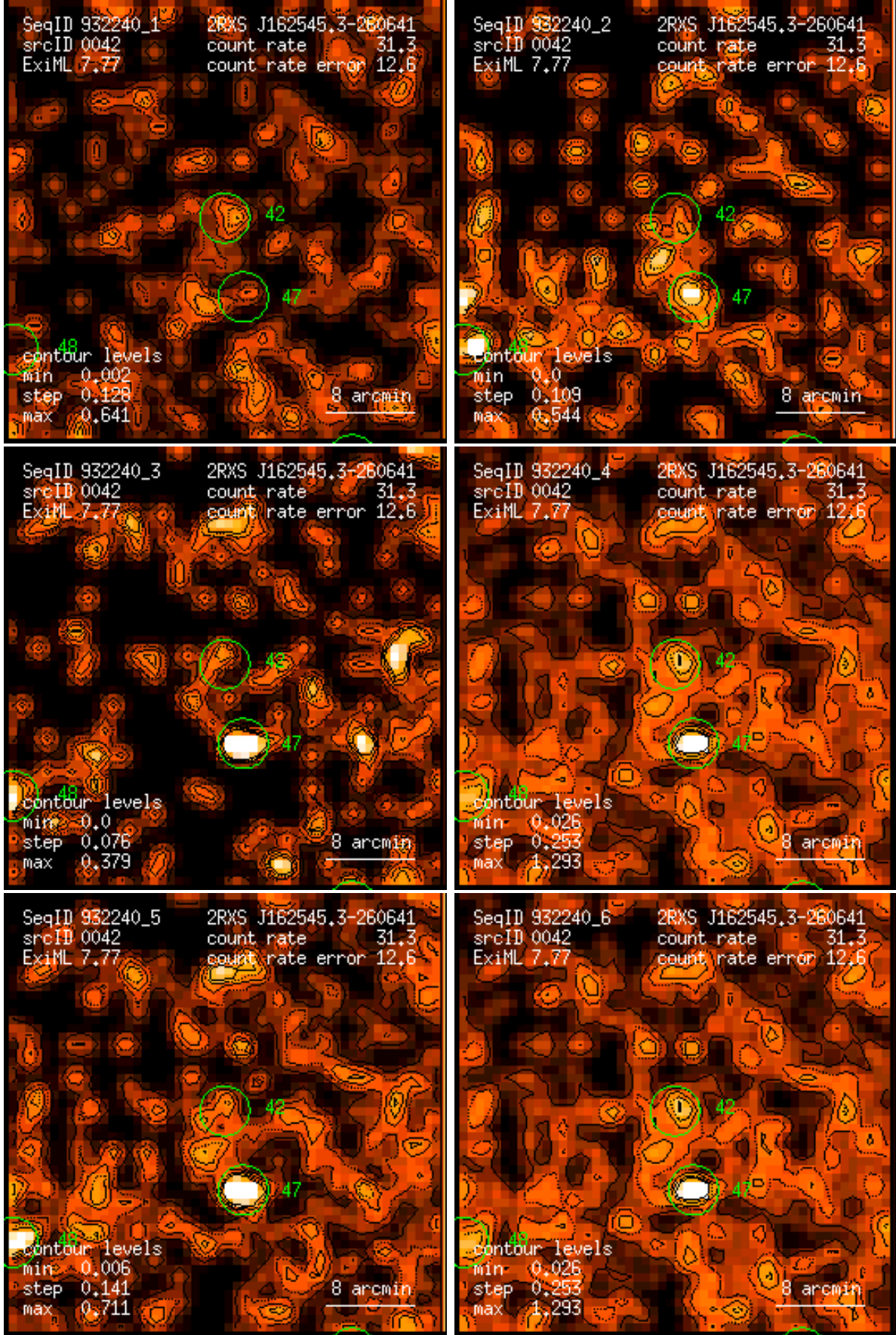
Figure 42: RASS 932240: detection 0042: band rate images, Gaussian filter: (1) PSPC channels 11 – 41, (2) 52 – 90, (3) 91 – 201, (4) 11 – 235, (5) 52 – 201, (6) 11 – 201. Broad band rates in counts/ks. Band rate contour levels in counts/ks/arcmin 2 .
