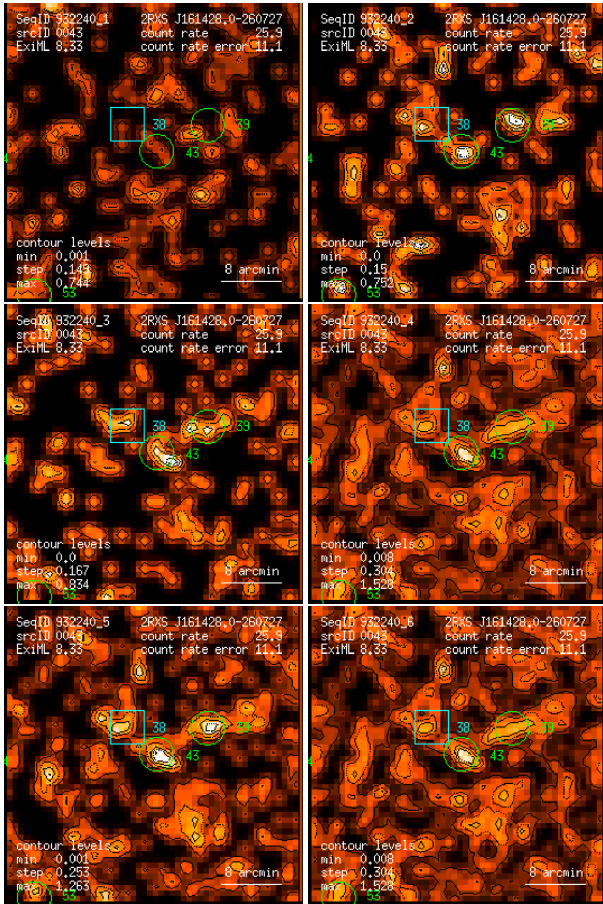
Figure 43: RASS 932240: detection 0043: band rate images, Gaussian filter: (1) PSPC channels 11 – 41, (2) 52 – 90, (3) 91 – 201, (4) 11 – 235, (5) 52 – 201, (6) 11 – 201. Broad band rates in counts/ks. Band rate contour levels in counts/ks/arcmin 2 .
