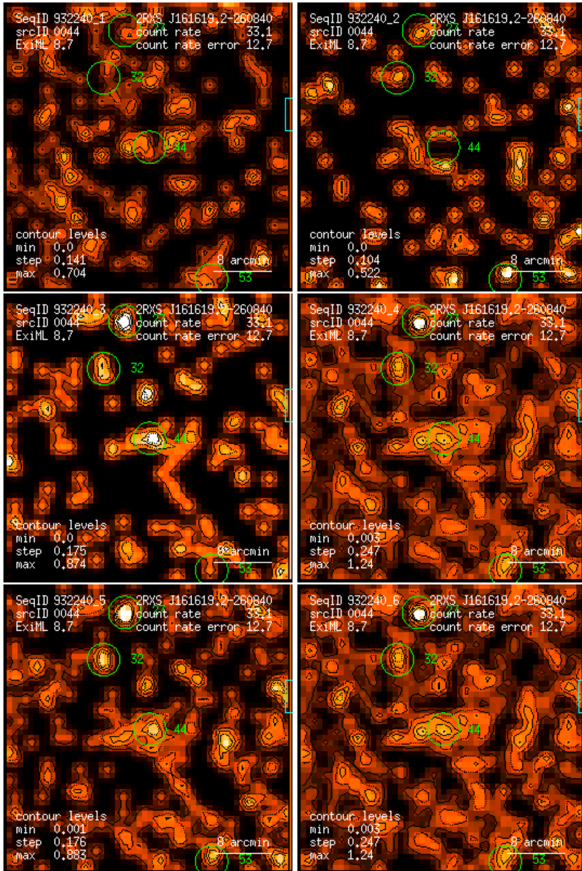
Figure 44: RASS 932240: detection 0044: band rate images, Gaussian filter: (1) PSPC channels 11 – 41, (2) 52 – 90, (3) 91 – 201, (4) 11 – 235, (5) 52 – 201, (6) 11 – 201. Broad band rates in counts/ks. Band rate contour levels in counts/ks/arcmin 2 .
