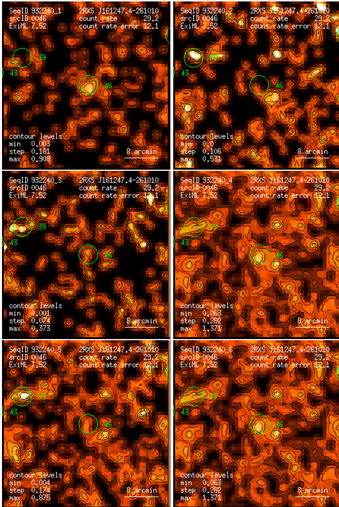
Figure 46: RASS 932240: detection 0046: band rate images, Gaussian filter: (1) PSPC channels 11 – 41, (2) 52 – 90, (3) 91 – 201, (4) 11 – 235, (5) 52 – 201, (6) 11 – 201. Broad band rates in counts/ks. Band rate contour levels in counts/ks/arcmin 2 .
