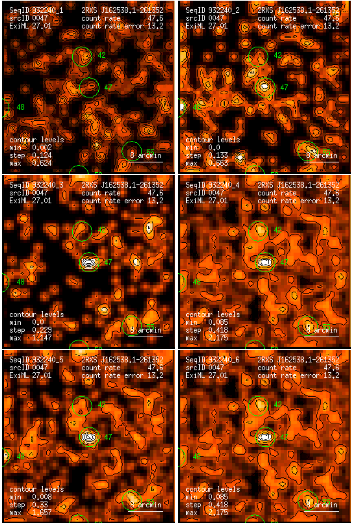
Figure 47: RASS 932240: detection 0047: band rate images, Gaussian filter: (1) PSPC channels 11 – 41, (2) 52 – 90, (3) 91 – 201, (4) 11 – 235, (5) 52 – 201, (6) 11 – 201. Broad band rates in counts/ks. Band rate contour levels in counts/ks/arcmin 2 .
