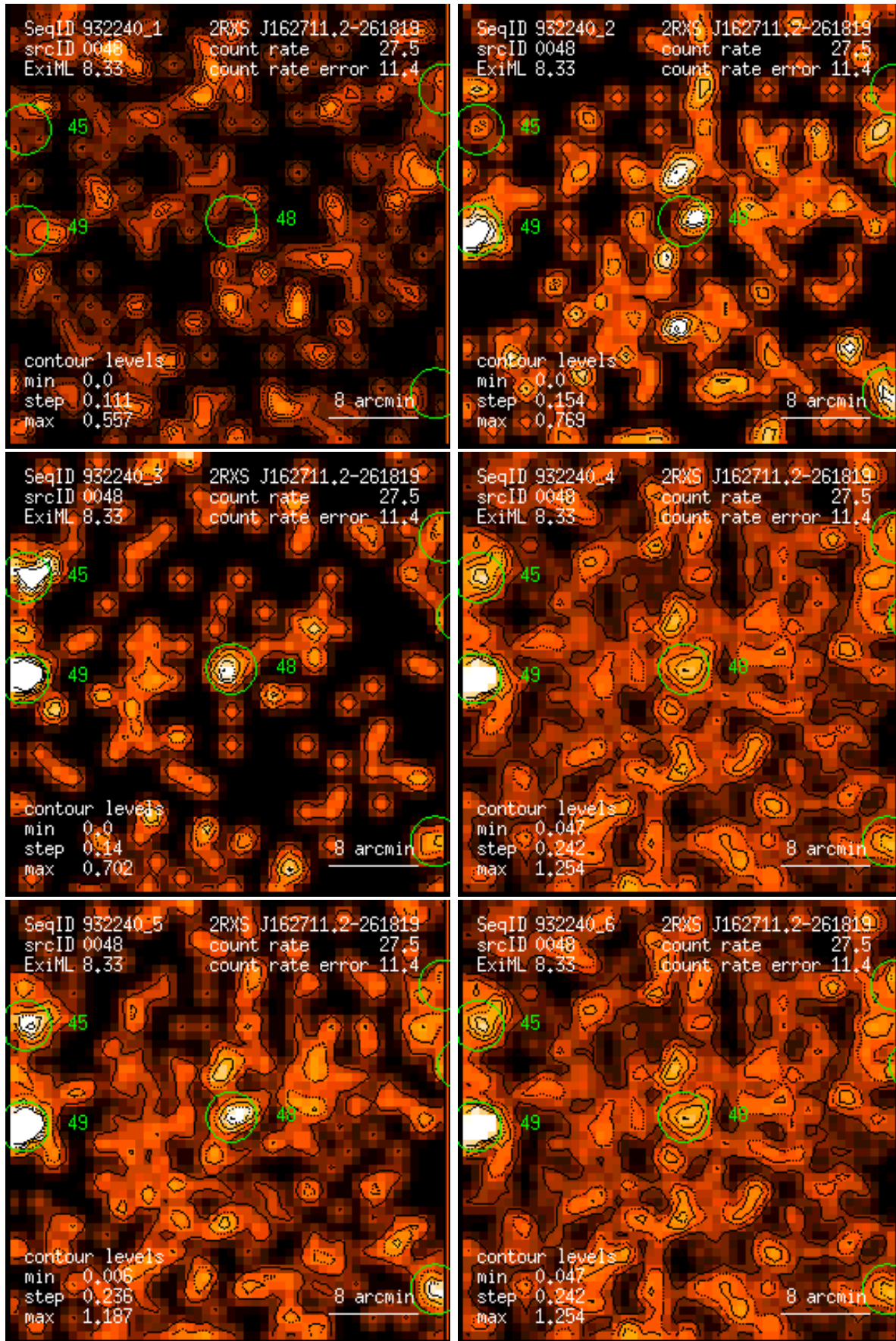
Figure 48: RASS 932240: detection 0048: band rate images, Gaussian filter: (1) PSPC channels 11 – 41, (2) 52 – 90, (3) 91 – 201, (4) 11 – 235, (5) 52 – 201, (6) 11 – 201. Broad band rates in counts/ks. Band rate contour levels in counts/ks/arcmin 2 .
