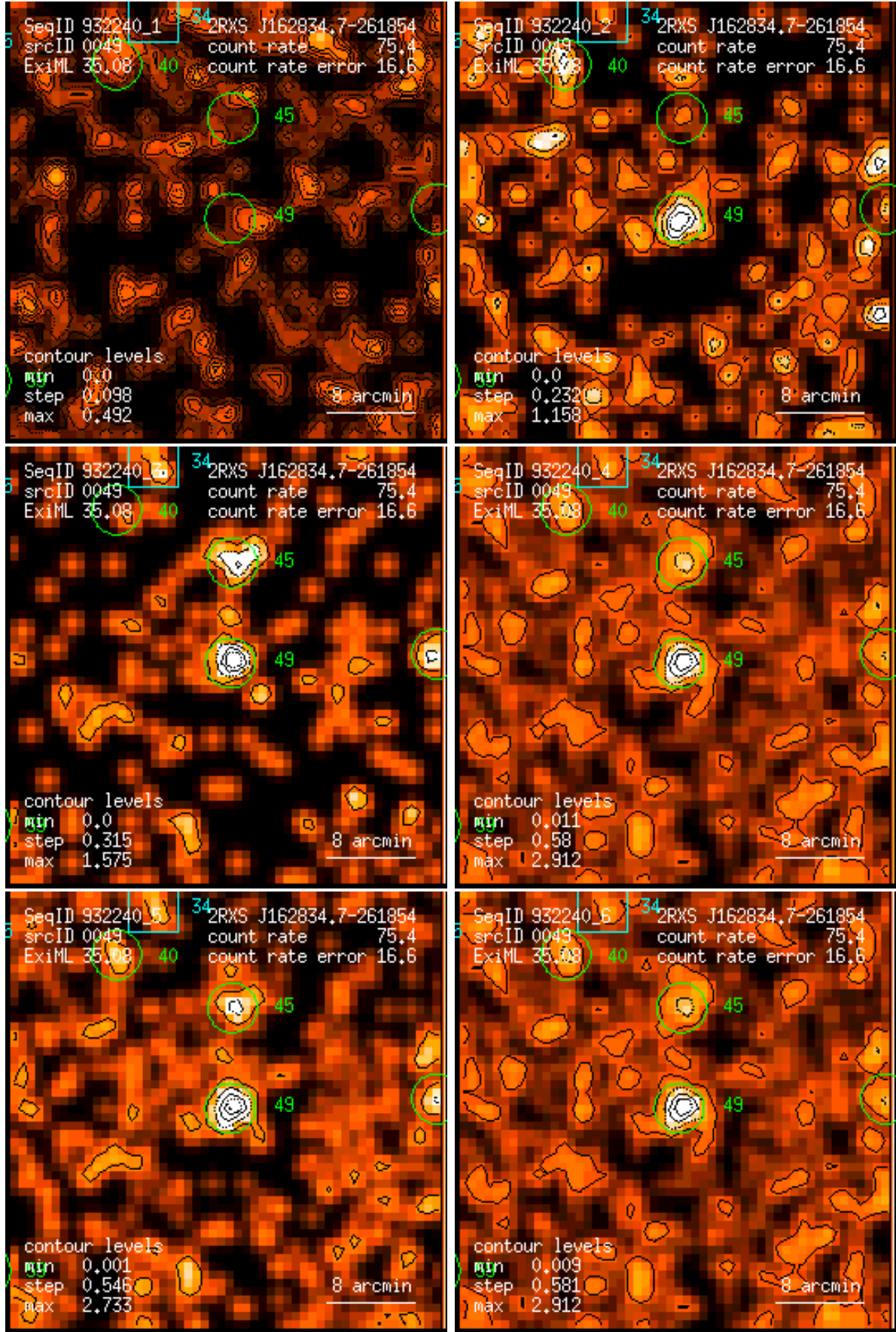
Figure 49: RASS 932240: detection 0049: band rate images, Gaussian filter: (1) PSPC channels 11 – 41, (2) 52 – 90, (3) 91 – 201, (4) 11 – 235, (5) 52 – 201, (6) 11 – 201. Broad band rates in counts/ks. Band rate contour levels in counts/ks/arcmin 2 .
