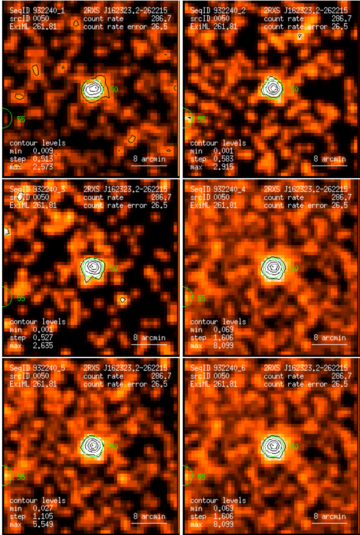
Figure 50: RASS 932240: detection 0050: band rate images, Gaussian filter: (1) PSPC channels 11 – 41, (2) 52 – 90, (3) 91 – 201, (4) 11 – 235, (5) 52 – 201, (6) 11 – 201. Broad band rates in counts/ks. Band rate contour levels in counts/ks/arcmin 2 .
