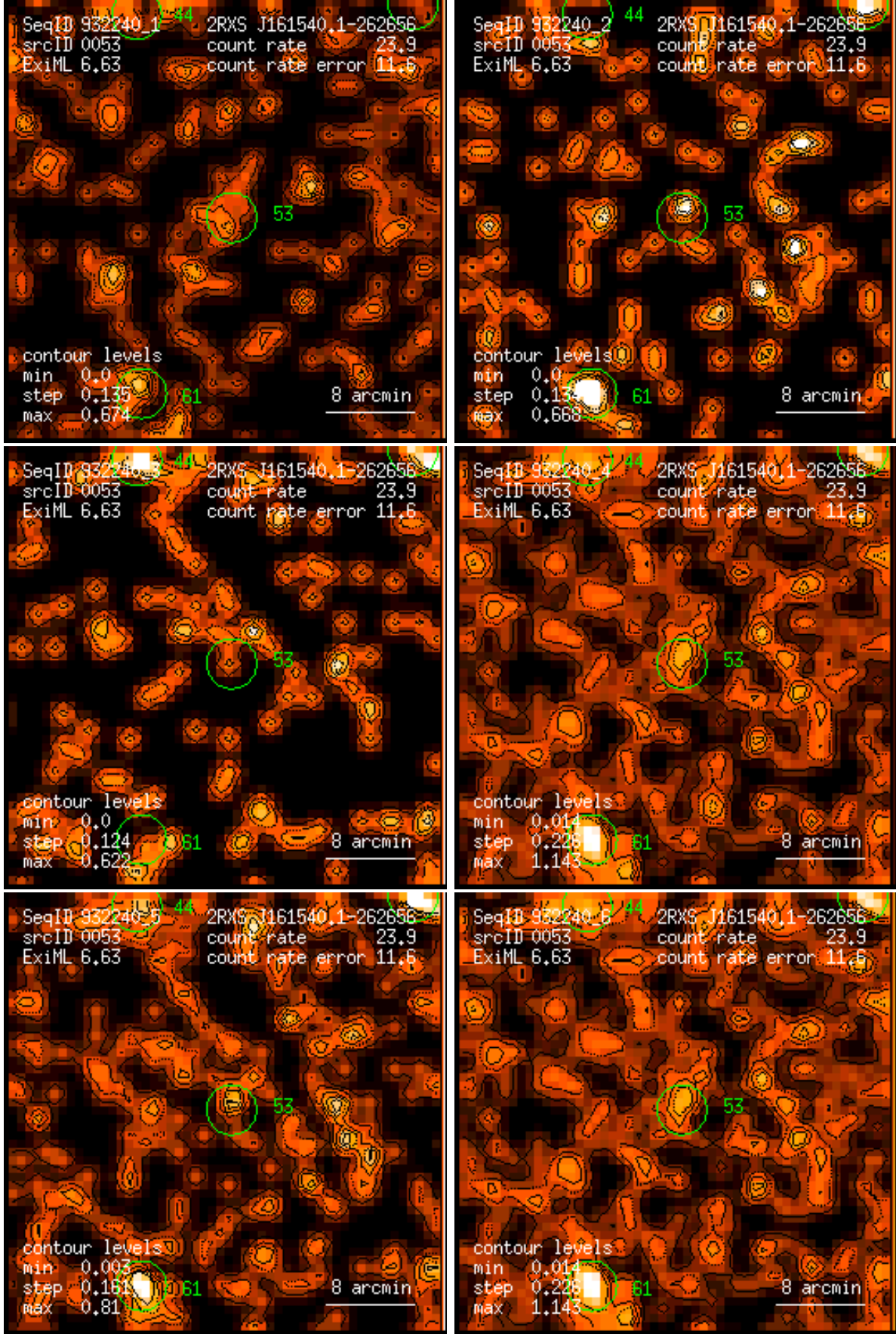
Figure 53: RASS 932240: detection 0053: band rate images, Gaussian filter: (1) PSPC channels 11 – 41, (2) 52 – 90, (3) 91 – 201, (4) 11 – 235, (5) 52 – 201, (6) 11 – 201. Broad band rates in counts/ks. Band rate contour levels in counts/ks/arcmin 2 .
