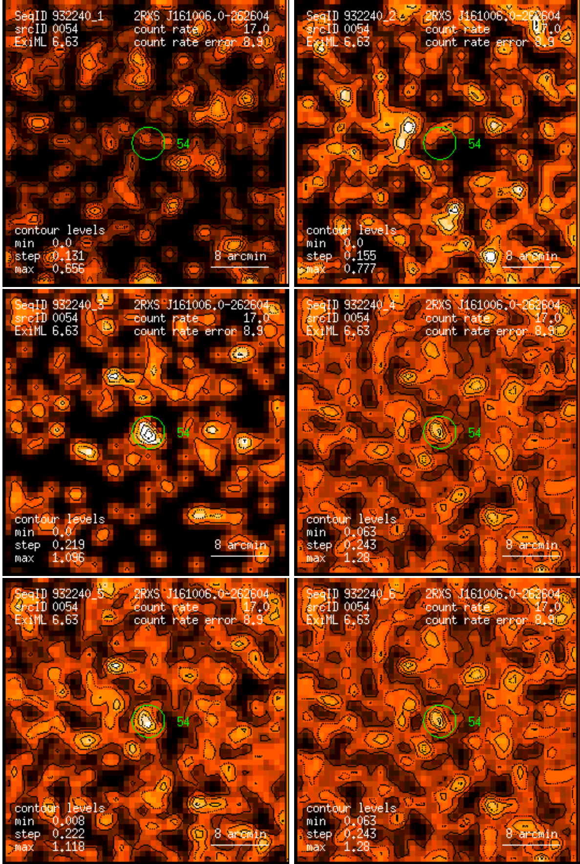
Figure 54: RASS 932240: detection 0054: band rate images, Gaussian filter: (1) PSPC channels 11 – 41, (2) 52 – 90, (3) 91 – 201, (4) 11 – 235, (5) 52 – 201, (6) 11 – 201. Broad band rates in counts/ks. Band rate contour levels in counts/ks/arcmin 2 .
