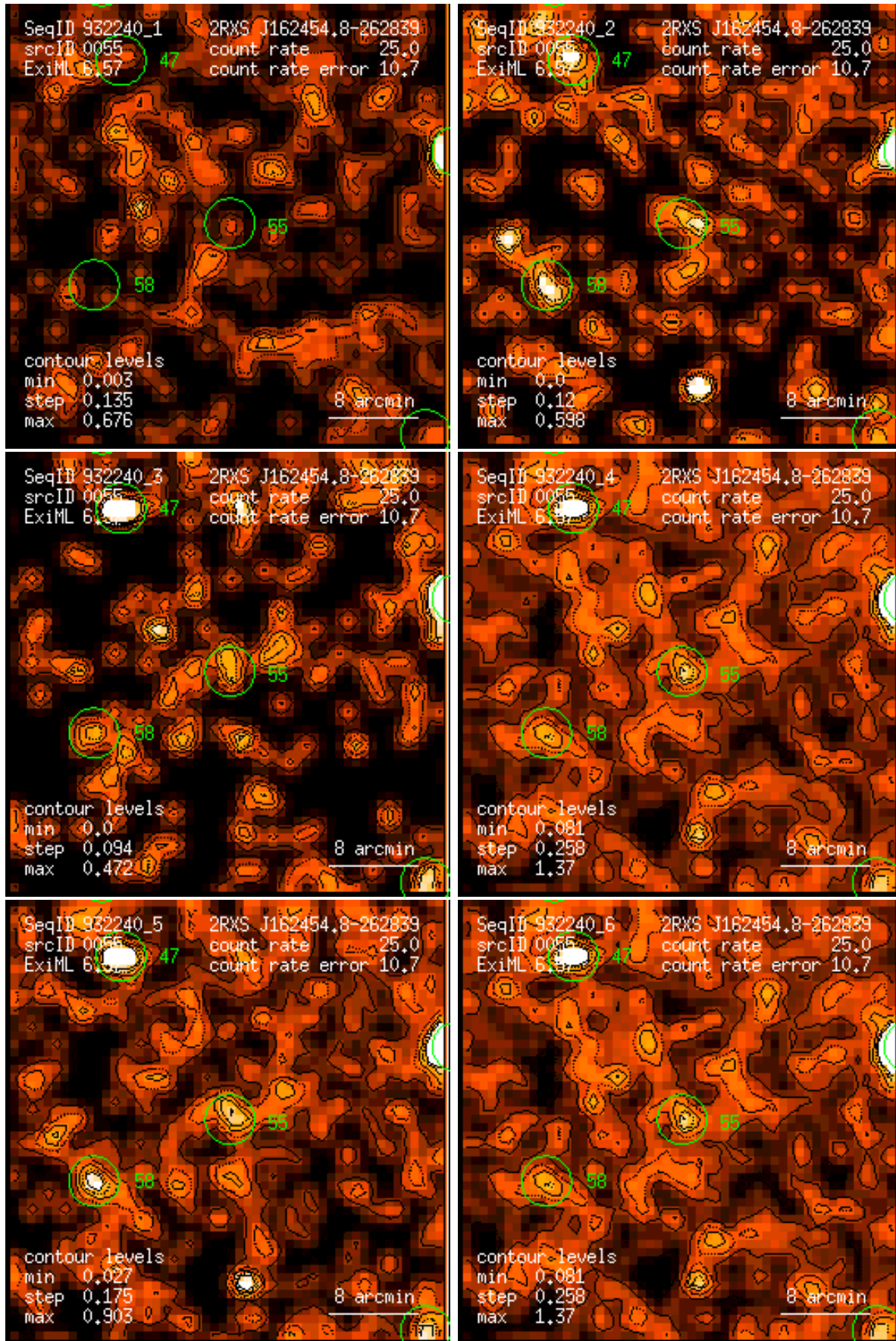
Figure 55: RASS 932240: detection 0055: band rate images, Gaussian filter: (1) PSPC channels 11 – 41, (2) 52 – 90, (3) 91 – 201, (4) 11 – 235, (5) 52 – 201, (6) 11 – 201. Broad band rates in counts/ks. Band rate contour levels in counts/ks/arcmin 2 .
