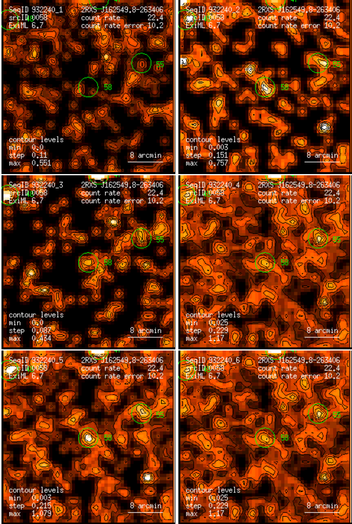
Figure 58: RASS 932240: detection 0058: band rate images, Gaussian filter: (1) PSPC channels 11 – 41, (2) 52 – 90, (3) 91 – 201, (4) 11 – 235, (5) 52 – 201, (6) 11 – 201. Broad band rates in counts/ks. Band rate contour levels in counts/ks/arcmin 2 .
