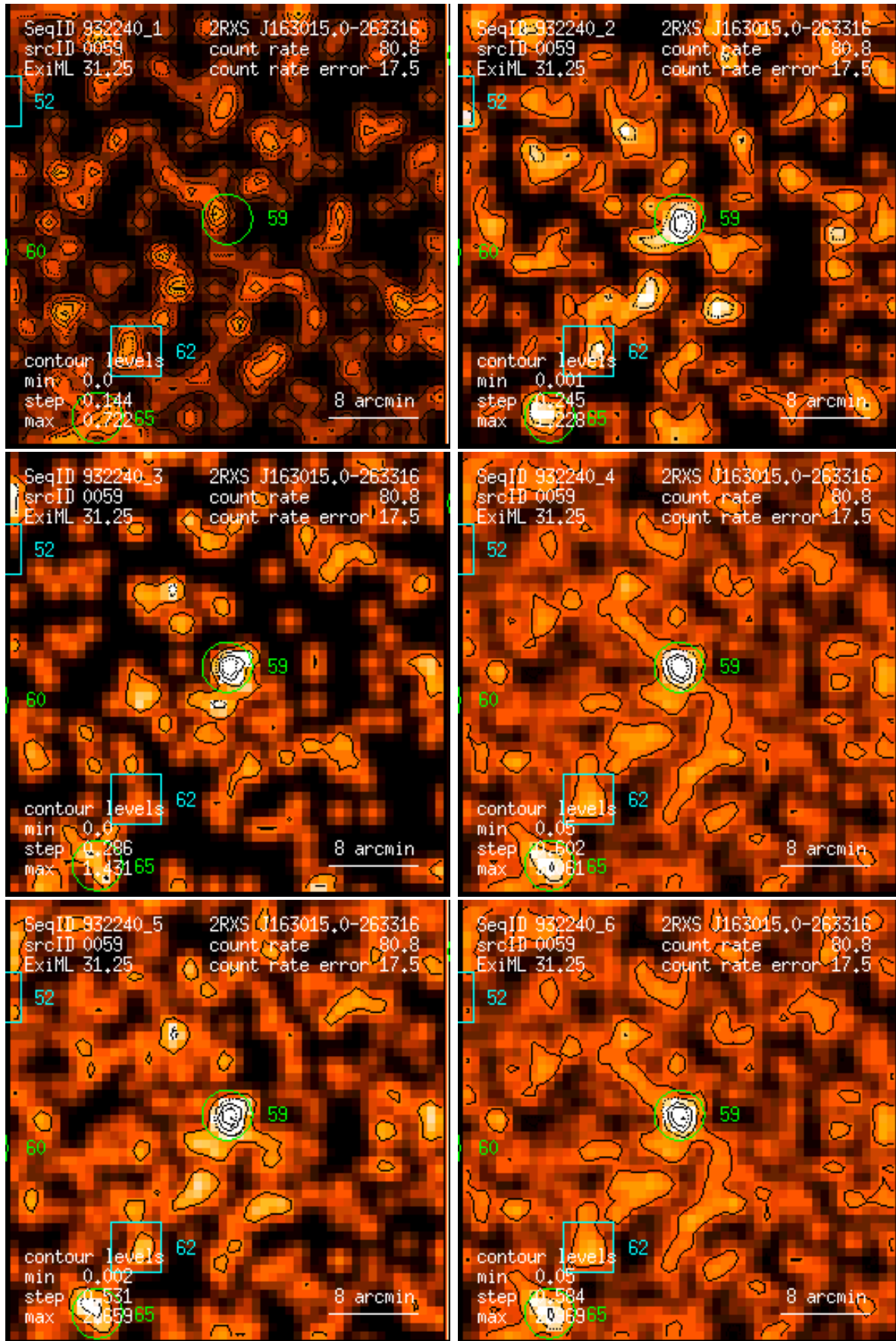
Figure 59: RASS 932240: detection 0059: band rate images, Gaussian filter: (1) PSPC channels 11 – 41, (2) 52 – 90, (3) 91 – 201, (4) 11 – 235, (5) 52 – 201, (6) 11 – 201. Broad band rates in counts/ks. Band rate contour levels in counts/ks/arcmin 2 .
