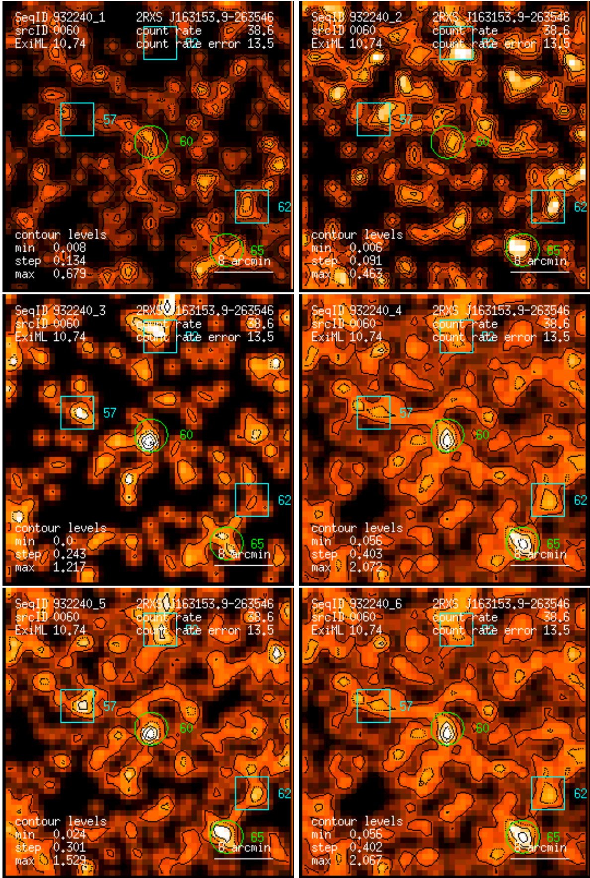
Figure 60: RASS 932240: detection 0060: band rate images, Gaussian filter: (1) PSPC channels 11 – 41, (2) 52 – 90, (3) 91 – 201, (4) 11 – 235, (5) 52 – 201, (6) 11 – 201. Broad band rates in counts/ks. Band rate contour levels in counts/ks/arcmin 2 .
