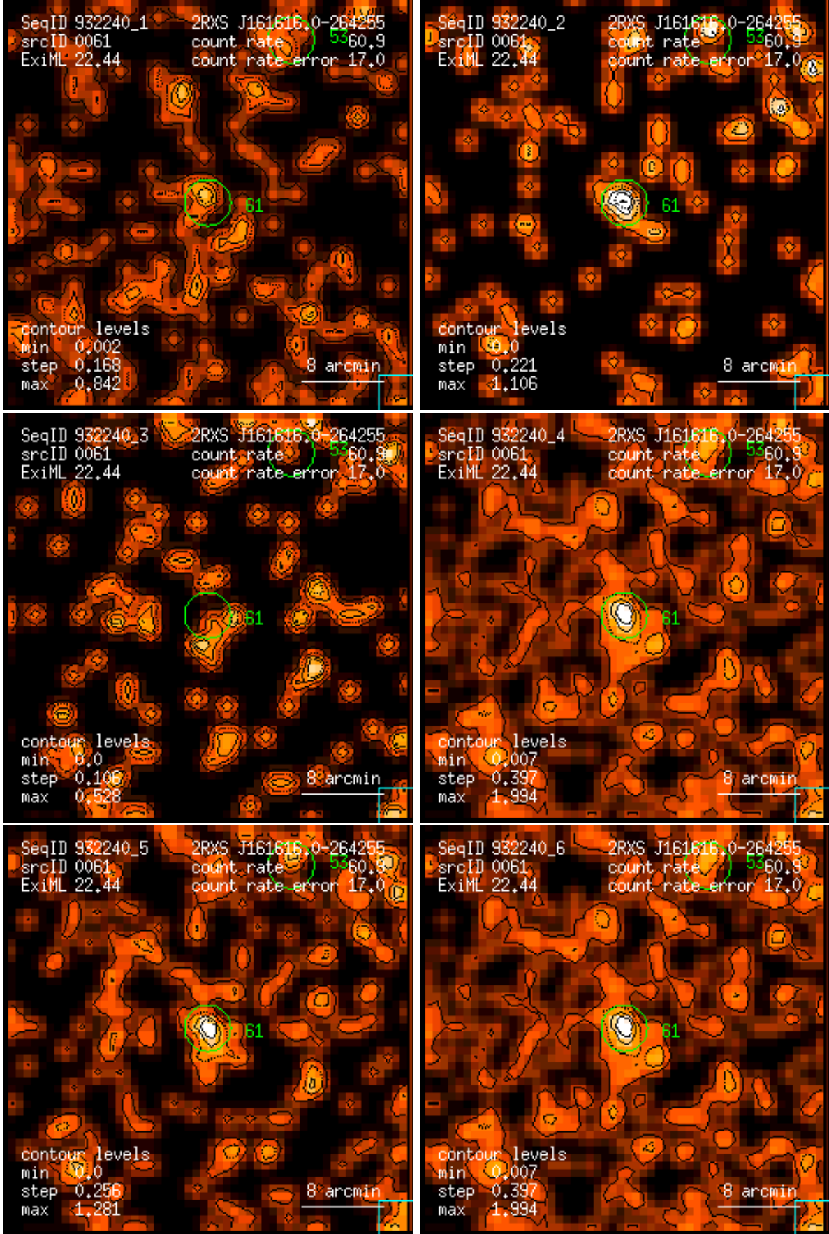
Figure 61: RASS 932240: detection 0061: band rate images, Gaussian filter: (1) PSPC channels 11 – 41, (2) 52 – 90, (3) 91 – 201, (4) 11 – 235, (5) 52 – 201, (6) 11 – 201. Broad band rates in counts/ks. Band rate contour levels in counts/ks/arcmin 2 .
