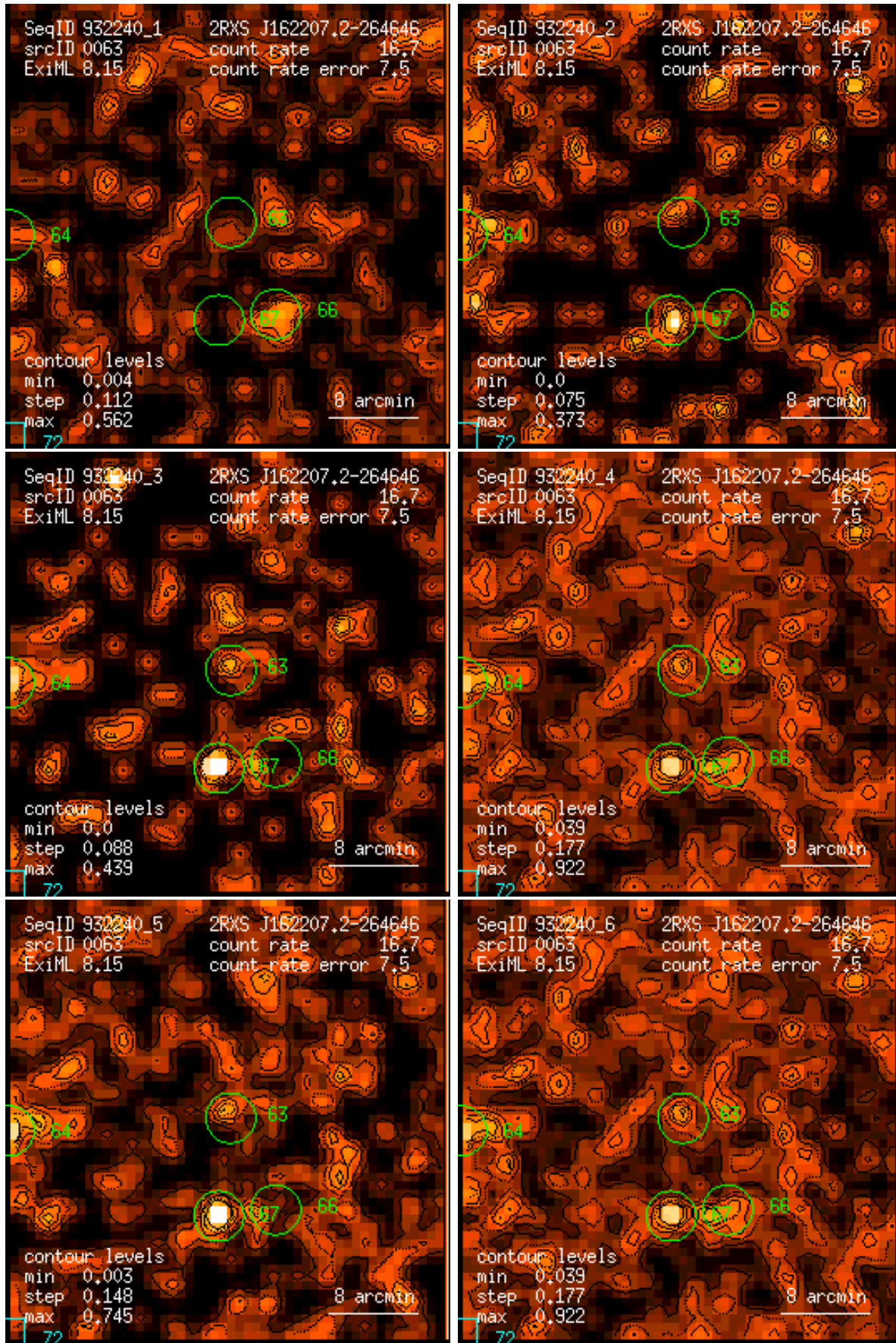
Figure 63: RASS 932240: detection 0063: band rate images, Gaussian filter: (1) PSPC channels 11 – 41, (2) 52 – 90, (3) 91 – 201, (4) 11 – 235, (5) 52 – 201, (6) 11 – 201. Broad band rates in counts/ks. Band rate contour levels in counts/ks/arcmin 2 .
