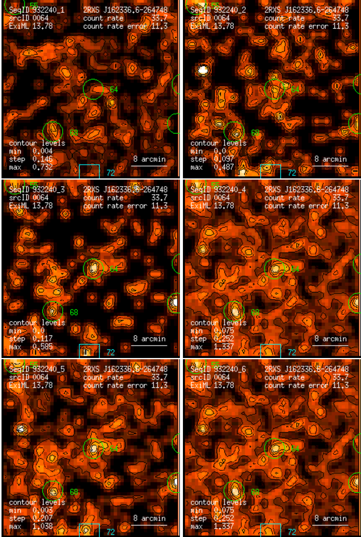
Figure 64: RASS 932240: detection 0064: band rate images, Gaussian filter: (1) PSPC channels 11 – 41, (2) 52 – 90, (3) 91 – 201, (4) 11 – 235, (5) 52 – 201, (6) 11 – 201. Broad band rates in counts/ks. Band rate contour levels in counts/ks/arcmin 2 .
