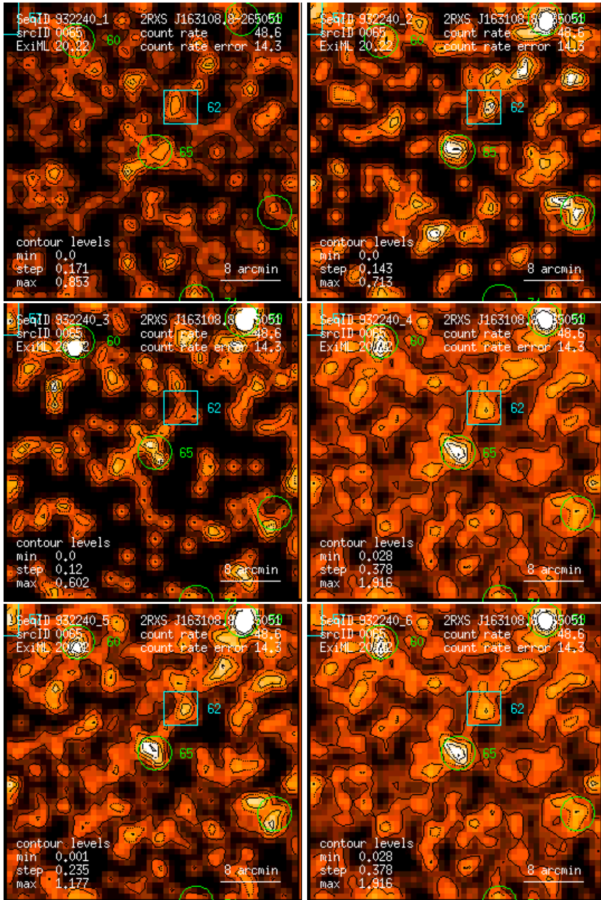
Figure 65: RASS 932240: detection 0065: band rate images, Gaussian filter: (1) PSPC channels 11 – 41, (2) 52 – 90, (3) 91 – 201, (4) 11 – 235, (5) 52 – 201, (6) 11 – 201. Broad band rates in counts/ks. Band rate contour levels in counts/ks/arcmin 2 .
