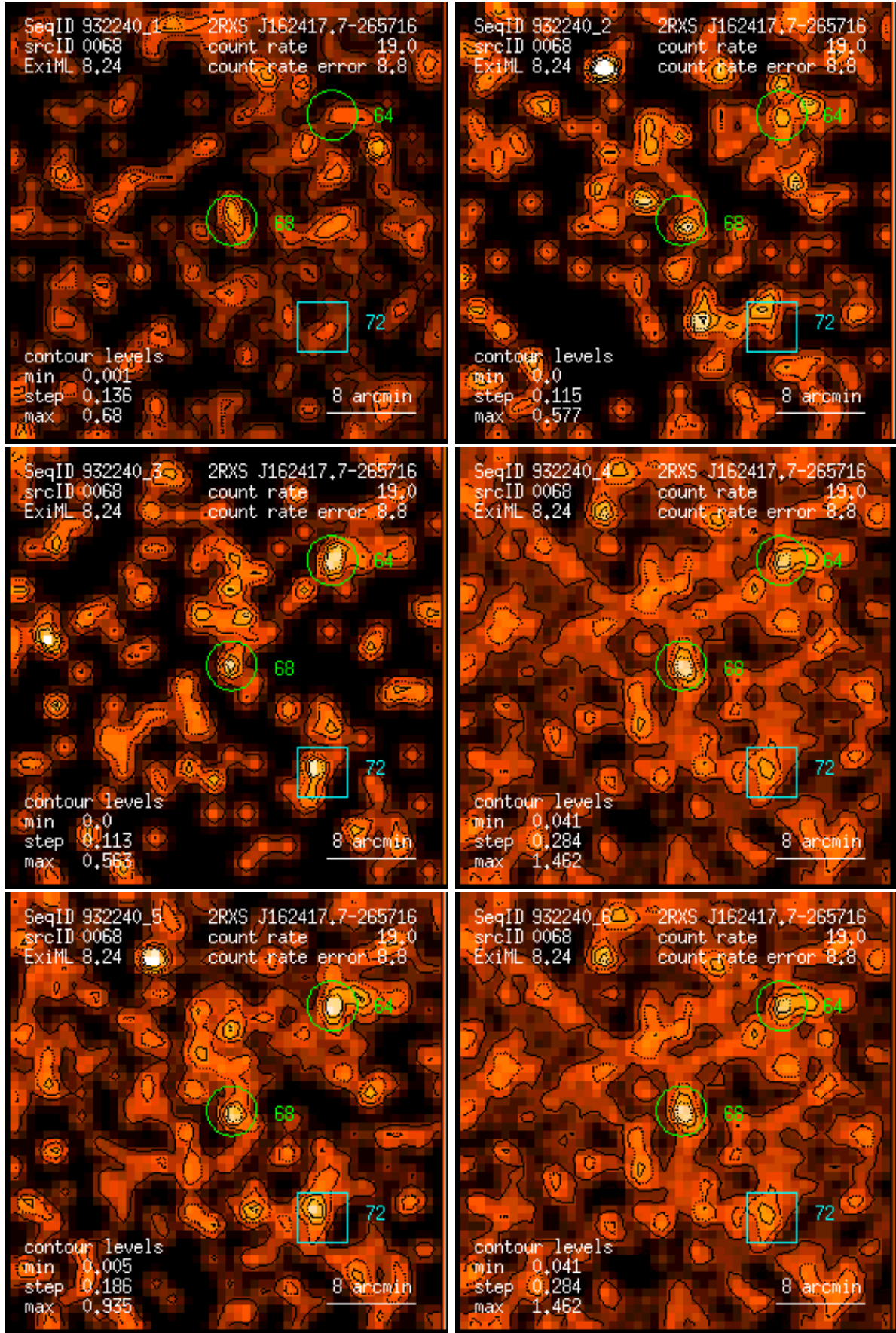
Figure 68: RASS 932240: detection 0068: band rate images, Gaussian filter: (1) PSPC channels 11 – 41, (2) 52 – 90, (3) 91 – 201, (4) 11 – 235, (5) 52 – 201, (6) 11 – 201. Broad band rates in counts/ks. Band rate contour levels in counts/ks/arcmin 2 .
