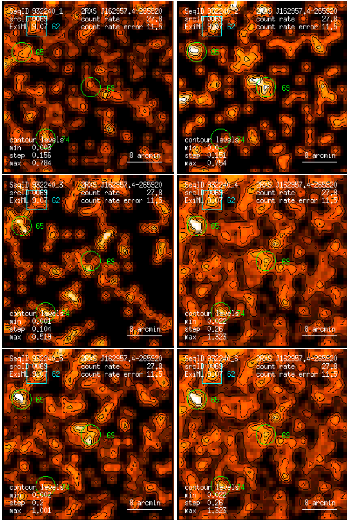
Figure 69: RASS 932240: detection 0069: band rate images, Gaussian filter: (1) PSPC channels 11 – 41, (2) 52 – 90, (3) 91 – 201, (4) 11 – 235, (5) 52 – 201, (6) 11 – 201. Broad band rates in counts/ks. Band rate contour levels in counts/ks/arcmin 2 .
