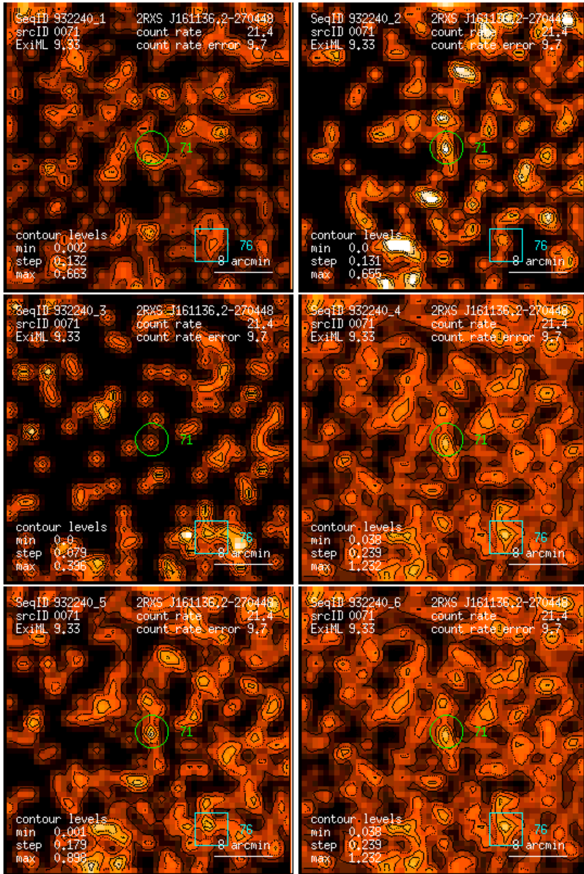
Figure 71: RASS 932240: detection 0071: band rate images, Gaussian filter: (1) PSPC channels 11 – 41, (2) 52 – 90, (3) 91 – 201, (4) 11 – 235, (5) 52 – 201, (6) 11 – 201. Broad band rates in counts/ks. Band rate contour levels in counts/ks/arcmin 2 .
