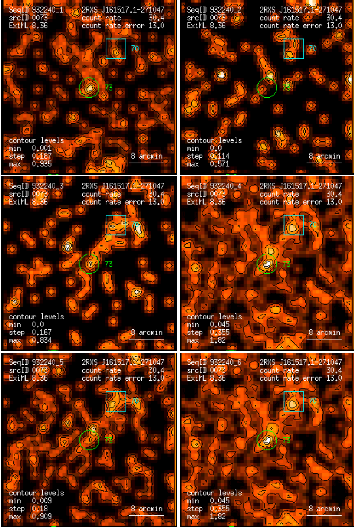
Figure 73: RASS 932240: detection 0073: band rate images, Gaussian filter: (1) PSPC channels 11 – 41, (2) 52 – 90, (3) 91 – 201, (4) 11 – 235, (5) 52 – 201, (6) 11 – 201. Broad band rates in counts/ks. Band rate contour levels in counts/ks/arcmin 2 .
