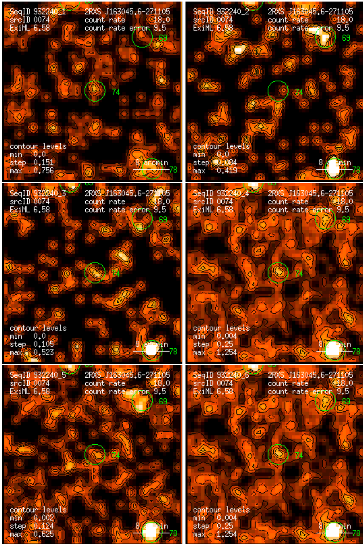
Figure 74: RASS 932240: detection 0074: band rate images, Gaussian filter: (1) PSPC channels 11 – 41, (2) 52 – 90, (3) 91 – 201, (4) 11 – 235, (5) 52 – 201, (6) 11 – 201. Broad band rates in counts/ks. Band rate contour levels in counts/ks/arcmin 2 .
