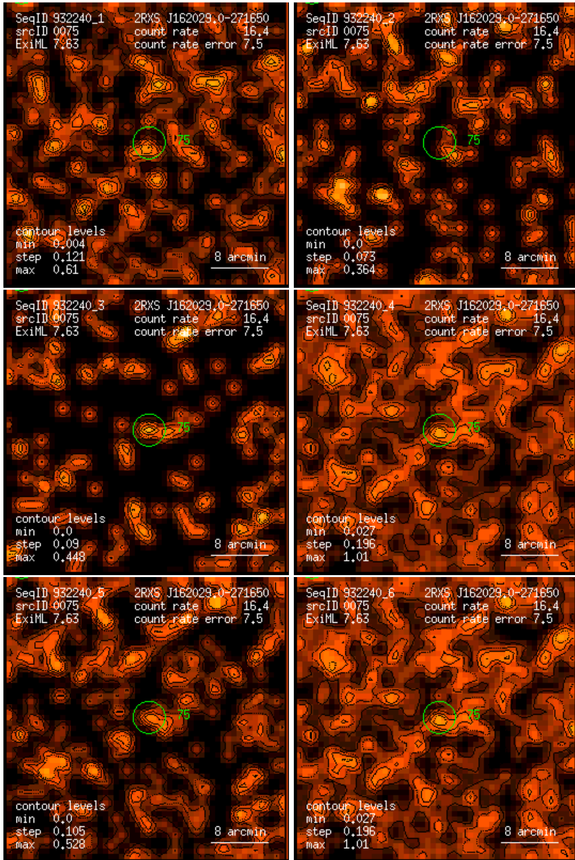
Figure 75: RASS 932240: detection 0075: band rate images, Gaussian filter: (1) PSPC channels 11 – 41, (2) 52 – 90, (3) 91 – 201, (4) 11 – 235, (5) 52 – 201, (6) 11 – 201. Broad band rates in counts/ks. Band rate contour levels in counts/ks/arcmin 2 .
