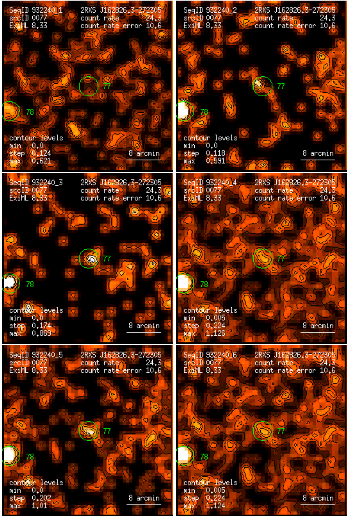
Figure 77: RASS 932240: detection 0077: band rate images, Gaussian filter: (1) PSPC channels 11 – 41, (2) 52 – 90, (3) 91 – 201, (4) 11 – 235, (5) 52 – 201, (6) 11 – 201. Broad band rates in counts/ks. Band rate contour levels in counts/ks/arcmin 2 .
