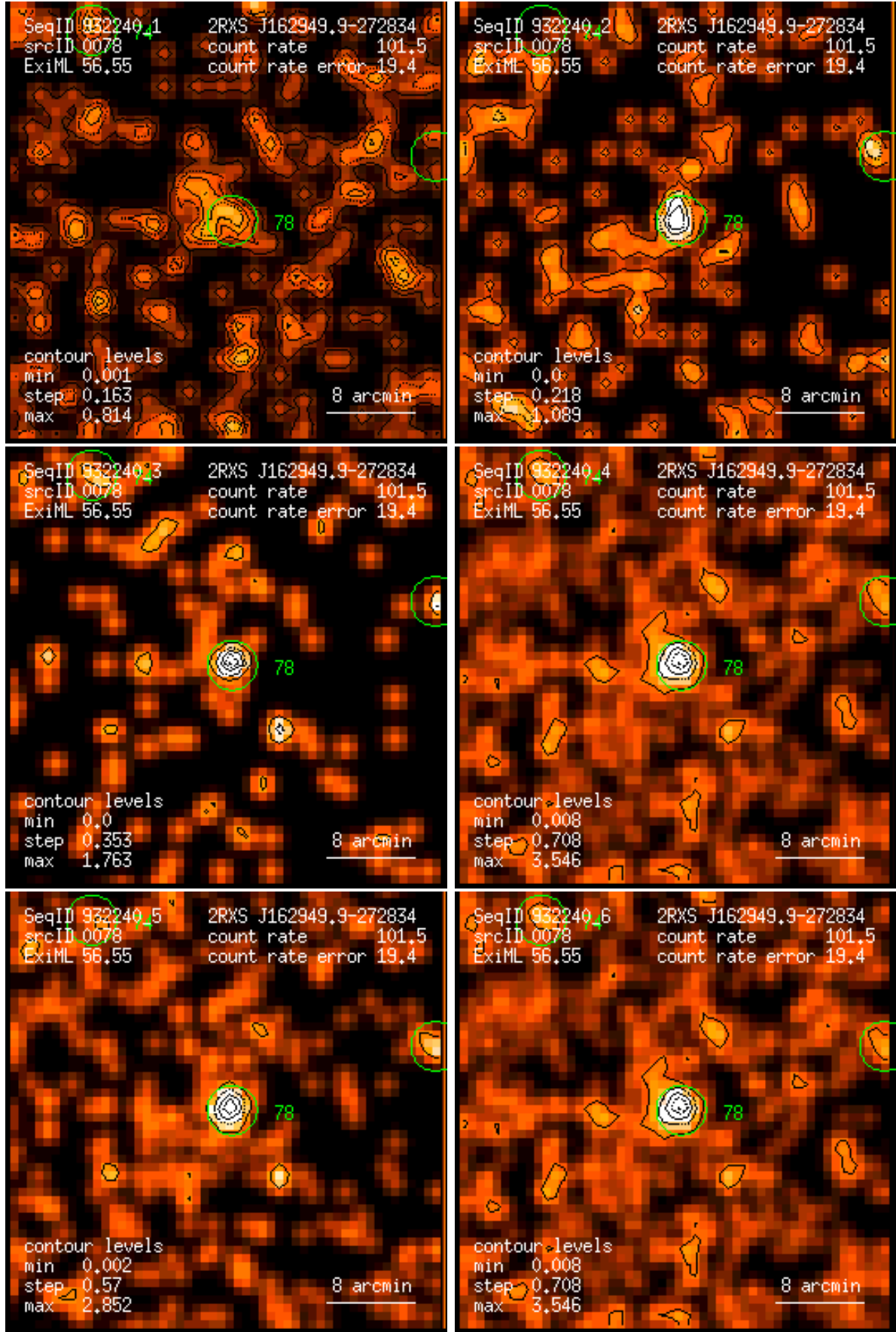
Figure 78: RASS 932240: detection 0078: band rate images, Gaussian filter: (1) PSPC channels 11 – 41, (2) 52 – 90, (3) 91 – 201, (4) 11 – 235, (5) 52 – 201, (6) 11 – 201. Broad band rates in counts/ks. Band rate contour levels in counts/ks/arcmin 2 .
