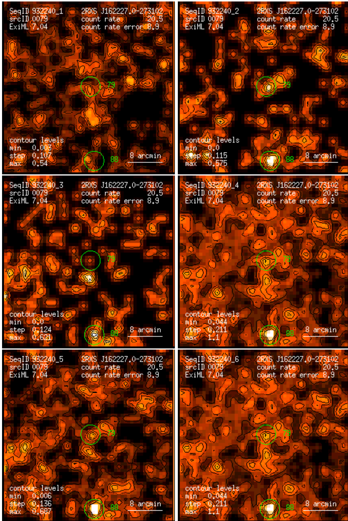
Figure 79: RASS 932240: detection 0079: band rate images, Gaussian filter: (1) PSPC channels 11 – 41, (2) 52 – 90, (3) 91 – 201, (4) 11 – 235, (5) 52 – 201, (6) 11 – 201. Broad band rates in counts/ks. Band rate contour levels in counts/ks/arcmin 2 .
