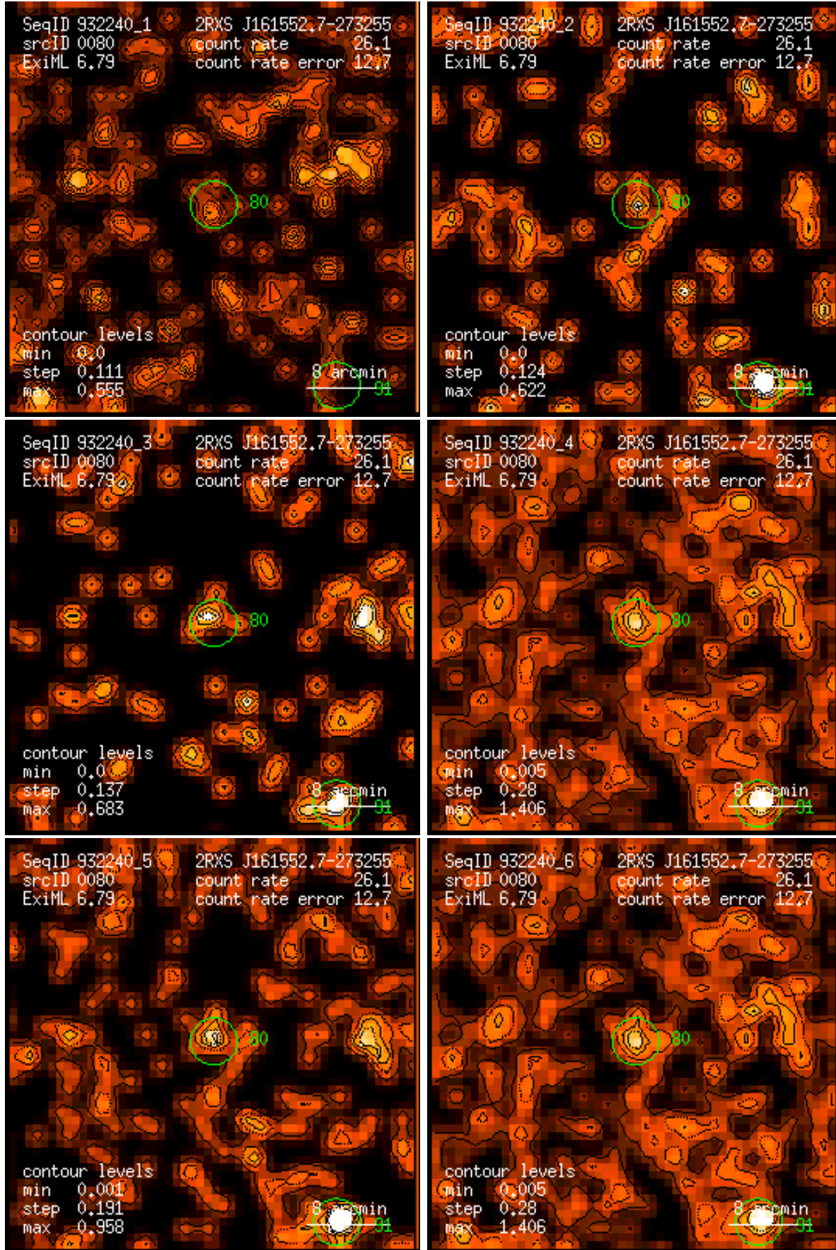
Figure 80: RASS 932240: detection 0080: band rate images, Gaussian filter: (1) PSPC channels 11 – 41, (2) 52 – 90, (3) 91 – 201, (4) 11 – 235, (5) 52 – 201, (6) 11 – 201. Broad band rates in counts/ks. Band rate contour levels in counts/ks/arcmin 2 .
