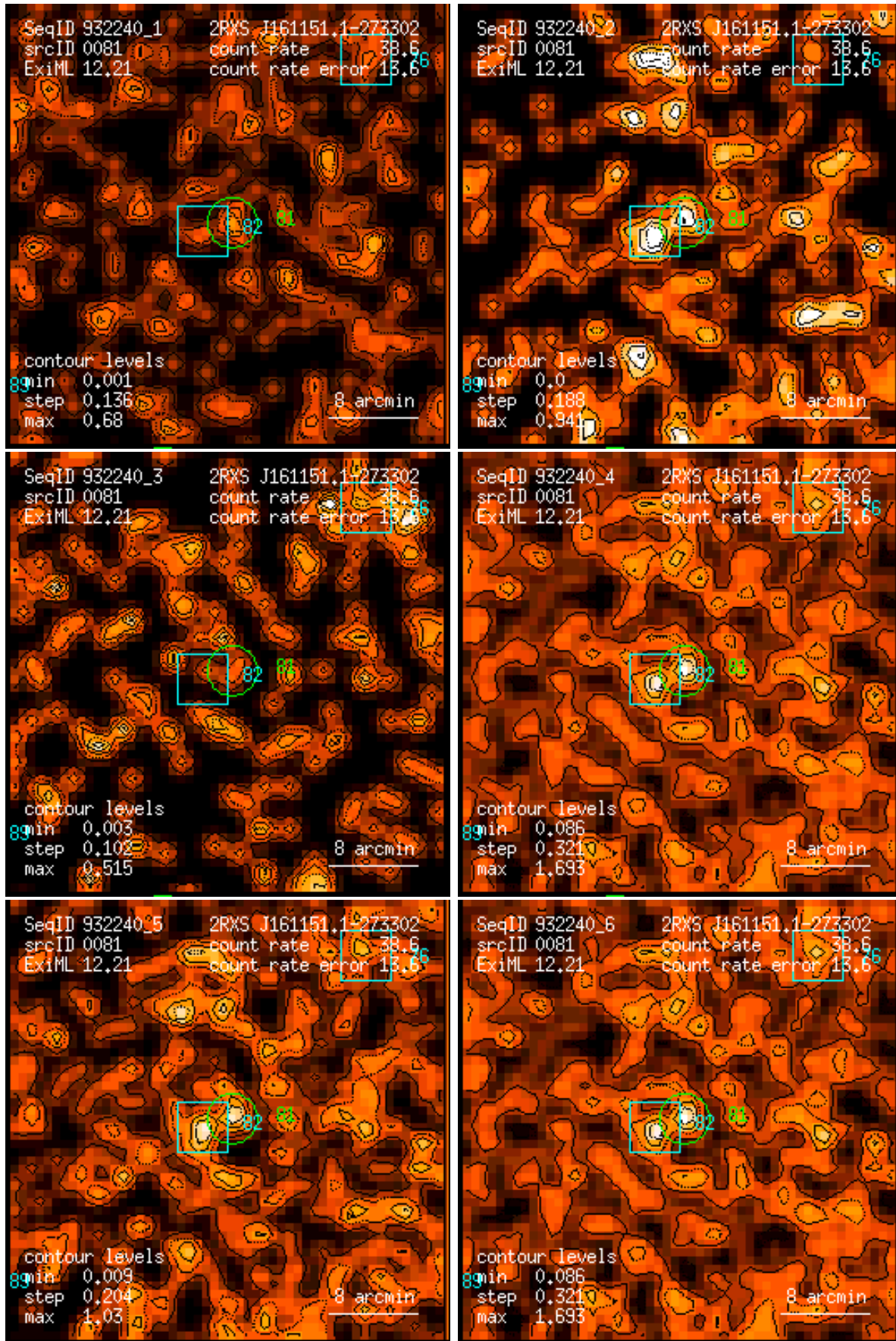
Figure 81: RASS 932240: detection 0081: band rate images, Gaussian filter: (1) PSPC channels 11 – 41, (2) 52 – 90, (3) 91 – 201, (4) 11 – 235, (5) 52 – 201, (6) 11 – 201. Broad band rates in counts/ks. Band rate contour levels in counts/ks/arcmin 2 .
