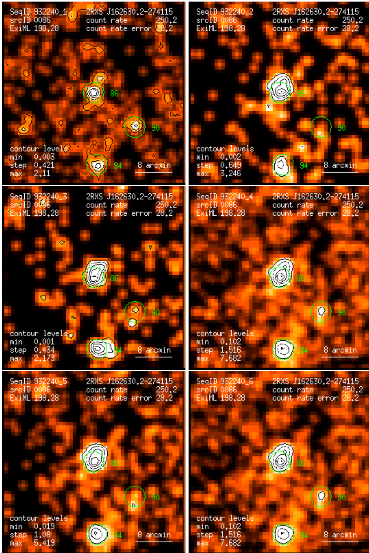
Figure 86: RASS 932240: detection 0086: band rate images, Gaussian filter: (1) PSPC channels 11 – 41, (2) 52 – 90, (3) 91 – 201, (4) 11 – 235, (5) 52 – 201, (6) 11 – 201. Broad band rates in counts/ks. Band rate contour levels in counts/ks/arcmin 2 .
