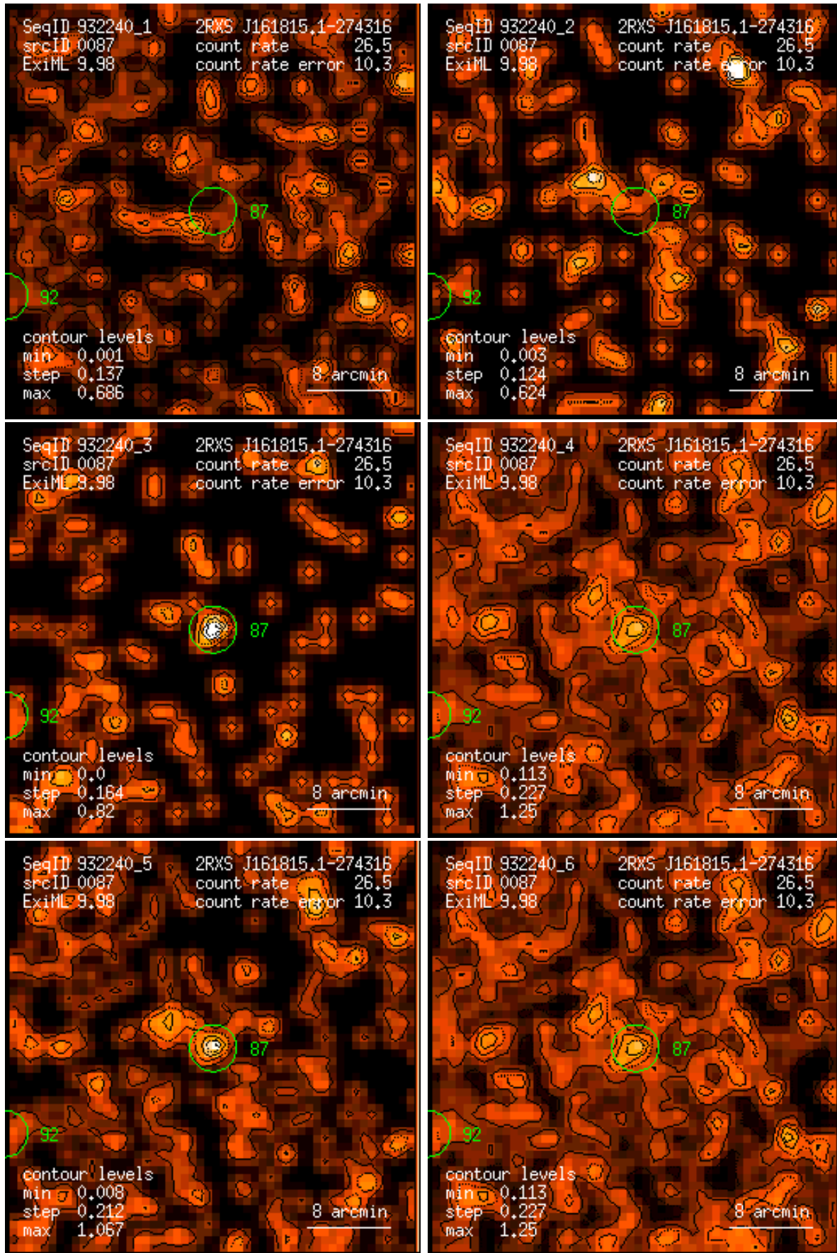
Figure 87: RASS 932240: detection 0087: band rate images, Gaussian filter: (1) PSPC channels 11 – 41, (2) 52 – 90, (3) 91 – 201, (4) 11 – 235, (5) 52 – 201, (6) 11 – 201. Broad band rates in counts/ks. Band rate contour levels in counts/ks/arcmin 2 .
