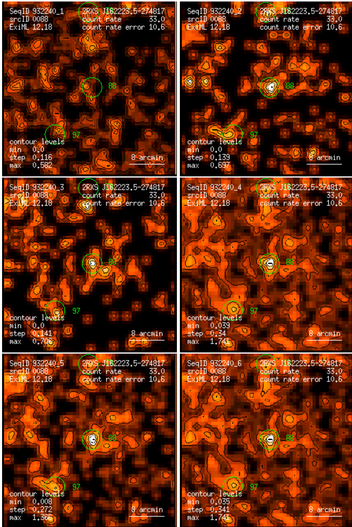
Figure 88: RASS 932240: detection 0088: band rate images, Gaussian filter: (1) PSPC channels 11 – 41, (2) 52 – 90, (3) 91 – 201, (4) 11 – 235, (5) 52 – 201, (6) 11 – 201. Broad band rates in counts/ks. Band rate contour levels in counts/ks/arcmin 2 .
