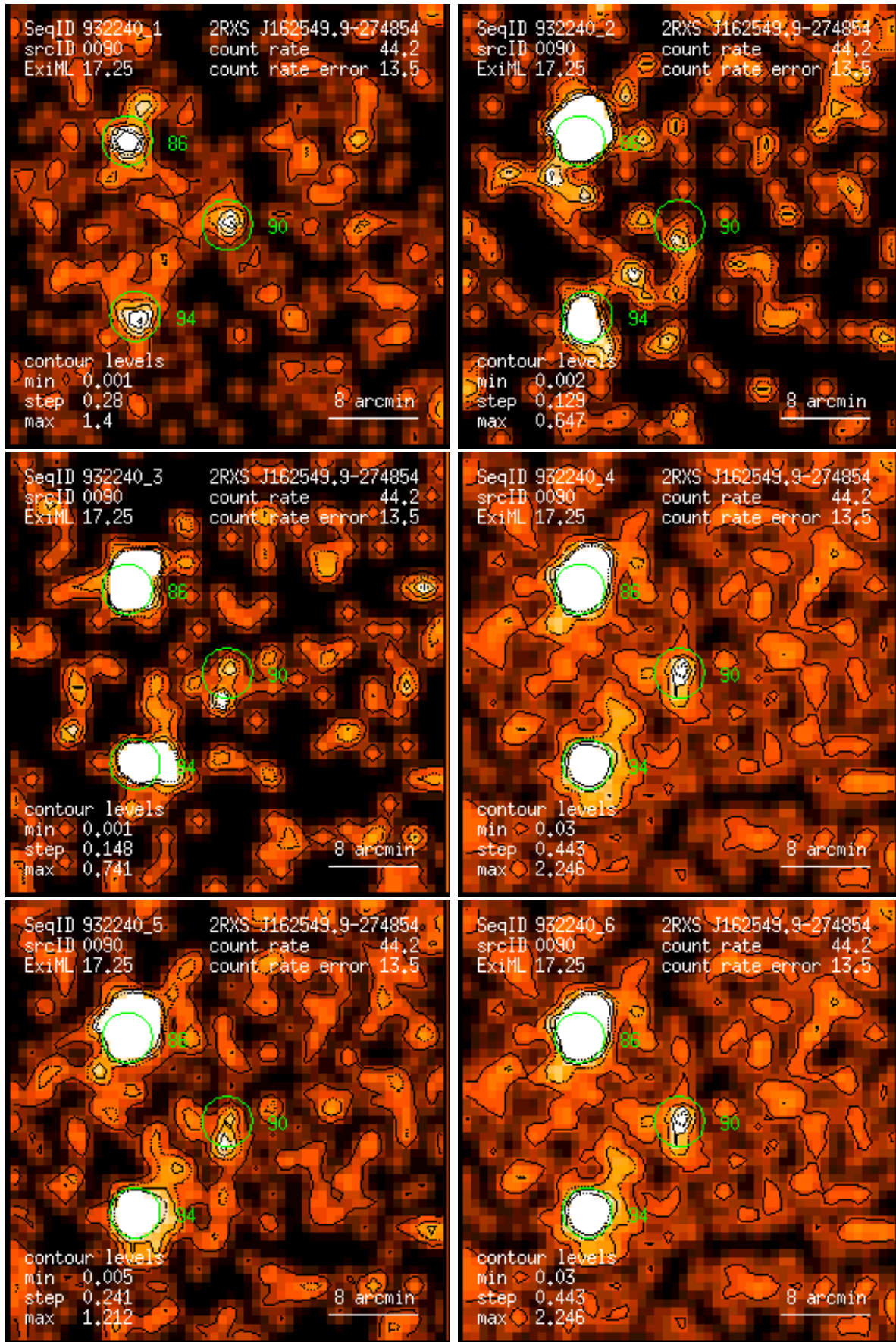
Figure 90: RASS 932240: detection 0090: band rate images, Gaussian filter: (1) PSPC channels 11 – 41, (2) 52 – 90, (3) 91 – 201, (4) 11 – 235, (5) 52 – 201, (6) 11 – 201. Broad band rates in counts/ks. Band rate contour levels in counts/ks/arcmin 2 .
