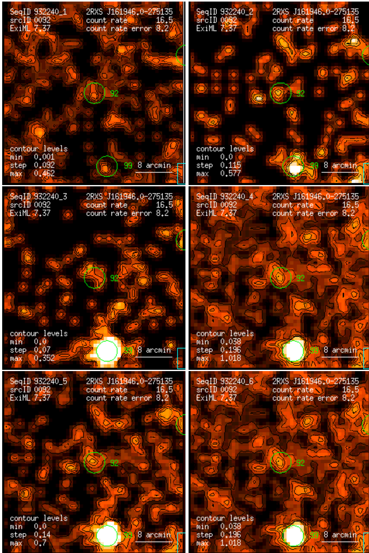
Figure 92: RASS 932240: detection 0092: band rate images, Gaussian filter: (1) PSPC channels 11 – 41, (2) 52 – 90, (3) 91 – 201, (4) 11 – 235, (5) 52 – 201, (6) 11 – 201. Broad band rates in counts/ks. Band rate contour levels in counts/ks/arcmin 2 .
