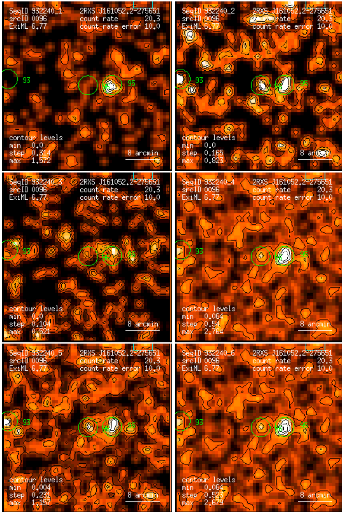
Figure 96: RASS 932240: detection 0096: band rate images, Gaussian filter: (1) PSPC channels 11 – 41, (2) 52 – 90, (3) 91 – 201, (4) 11 – 235, (5) 52 – 201, (6) 11 – 201. Broad band rates in counts/ks. Band rate contour levels in counts/ks/arcmin 2 .
