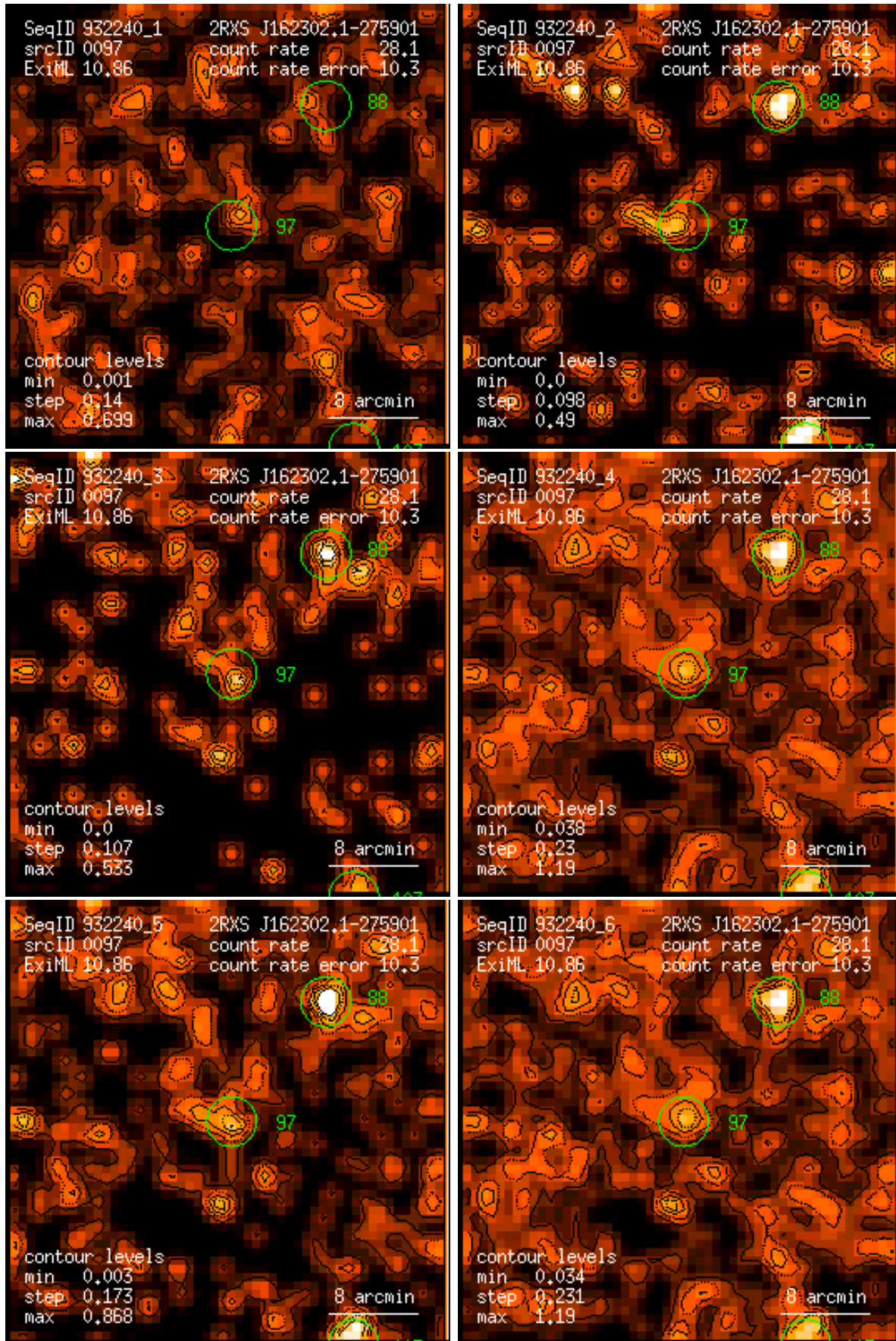
Figure 97: RASS 932240: detection 0097: band rate images, Gaussian filter: (1) PSPC channels 11 – 41, (2) 52 – 90, (3) 91 – 201, (4) 11 – 235, (5) 52 – 201, (6) 11 – 201. Broad band rates in counts/ks. Band rate contour levels in counts/ks/arcmin 2 .
