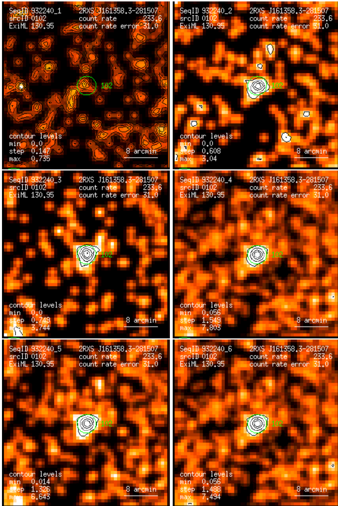
Figure 102: RASS 932240: detection 0102: band rate images, Gaussian filter: (1) PSPC channels 11 – 41, (2) 52 – 90, (3) 91 – 201, (4) 11 – 235, (5) 52 – 201, (6) 11 – 201. Broad band rates in counts/ks. Band rate contour levels in counts/ks/arcmin 2 .
