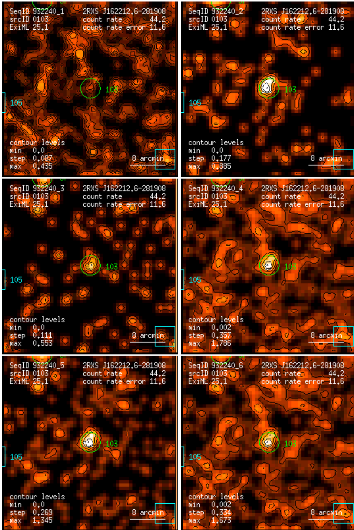
Figure 103: RASS 932240: detection 0103: band rate images, Gaussian filter: (1) PSPC channels 11 – 41, (2) 52 – 90, (3) 91 – 201, (4) 11 – 235, (5) 52 – 201, (6) 11 – 201. Broad band rates in counts/ks. Band rate contour levels in counts/ks/arcmin 2 .
