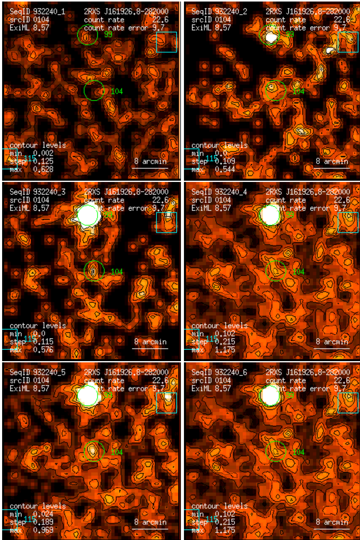
Figure 104: RASS 932240: detection 0104: band rate images, Gaussian filter: (1) PSPC channels 11 – 41, (2) 52 – 90, (3) 91 – 201, (4) 11 – 235, (5) 52 – 201, (6) 11 – 201. Broad band rates in counts/ks. Band rate contour levels in counts/ks/arcmin 2 .
