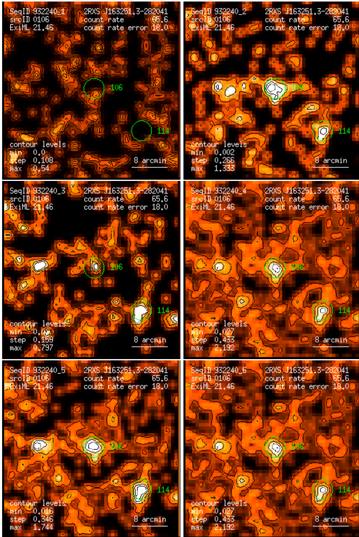
Figure 106: RASS 932240: detection 0106: band rate images, Gaussian filter: (1) PSPC channels 11 – 41, (2) 52 – 90, (3) 91 – 201, (4) 11 – 235, (5) 52 – 201, (6) 11 – 201. Broad band rates in counts/ks. Band rate contour levels in counts/ks/arcmin 2 .
