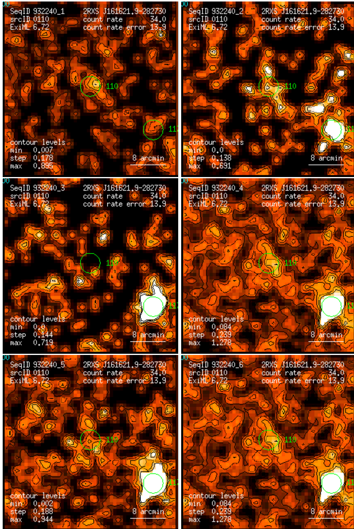
Figure 110: RASS 932240: detection 0110: band rate images, Gaussian filter: (1) PSPC channels 11 – 41, (2) 52 – 90, (3) 91 – 201, (4) 11 – 235, (5) 52 – 201, (6) 11 – 201. Broad band rates in counts/ks. Band rate contour levels in counts/ks/arcmin 2 .
