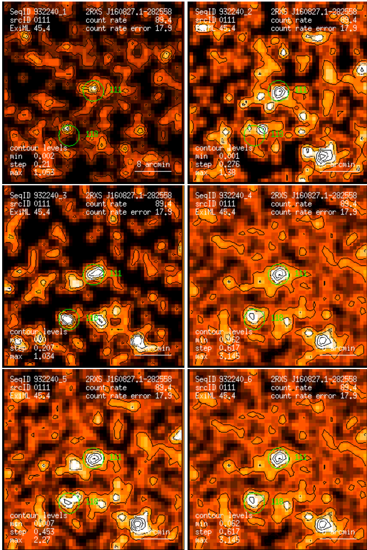
Figure 111: RASS 932240: detection 0111: band rate images, Gaussian filter: (1) PSPC channels 11 – 41, (2) 52 – 90, (3) 91 – 201, (4) 11 – 235, (5) 52 – 201, (6) 11 – 201. Broad band rates in counts/ks. Band rate contour levels in counts/ks/arcmin 2 .
