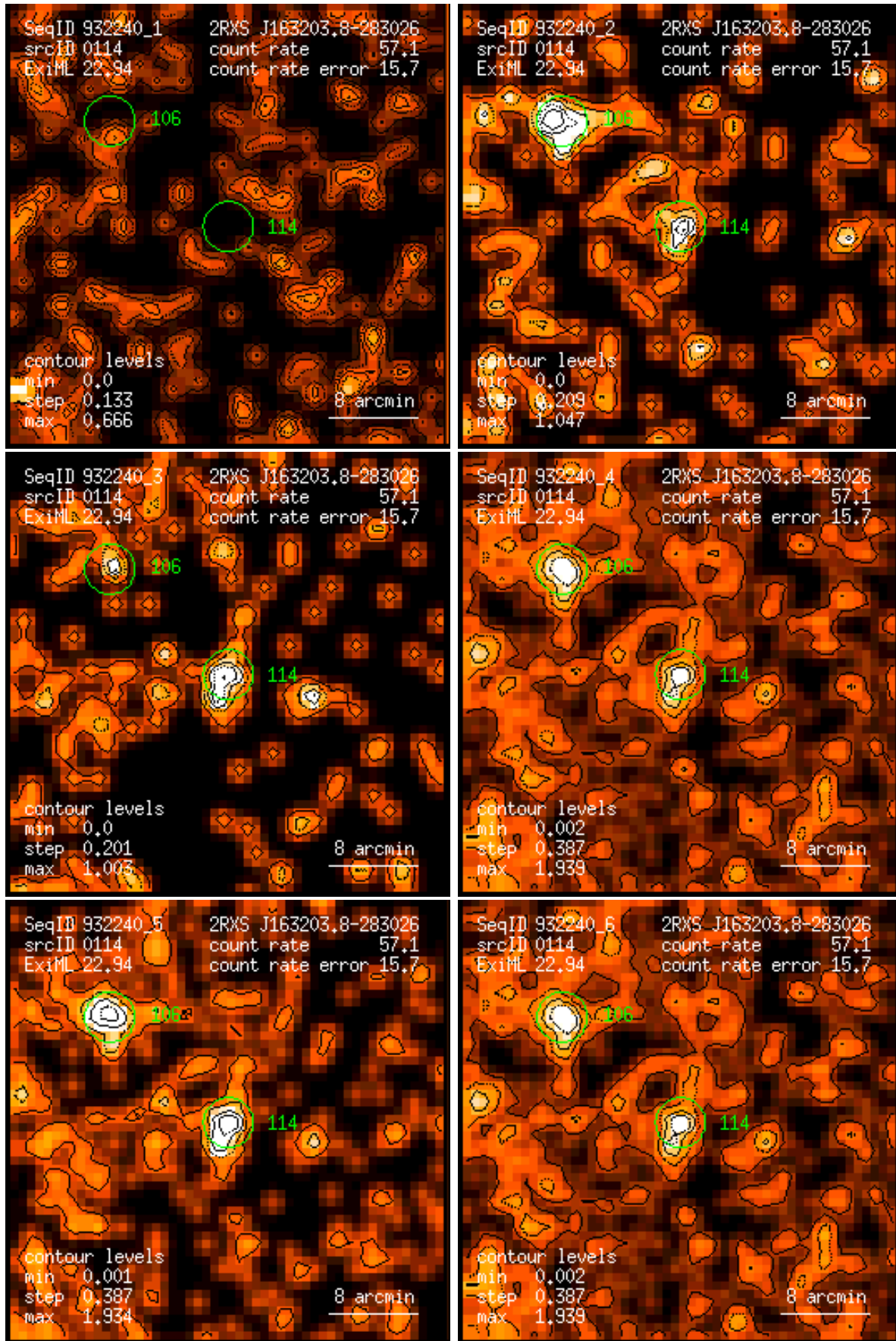
Figure 114: RASS 932240: detection 0114: band rate images, Gaussian filter: (1) PSPC channels 11 – 41, (2) 52 – 90, (3) 91 – 201, (4) 11 – 235, (5) 52 – 201, (6) 11 – 201. Broad band rates in counts/ks. Band rate contour levels in counts/ks/arcmin 2 .
