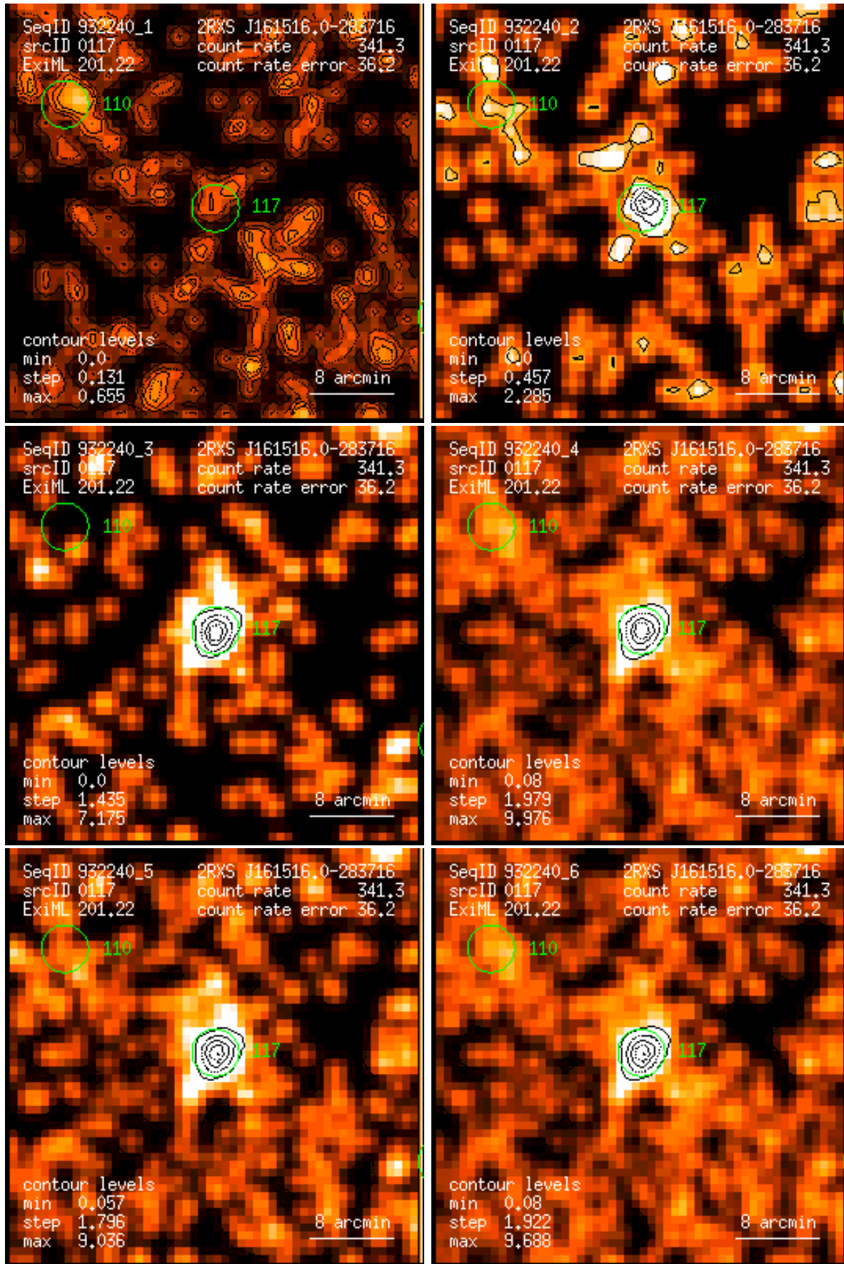
Figure 117: RASS 932240: detection 0117: band rate images, Gaussian filter: (1) PSPC channels 11 – 41, (2) 52 – 90, (3) 91 – 201, (4) 11 – 235, (5) 52 – 201, (6) 11 – 201. Broad band rates in counts/ks. Band rate contour levels in counts/ks/arcmin 2 .
