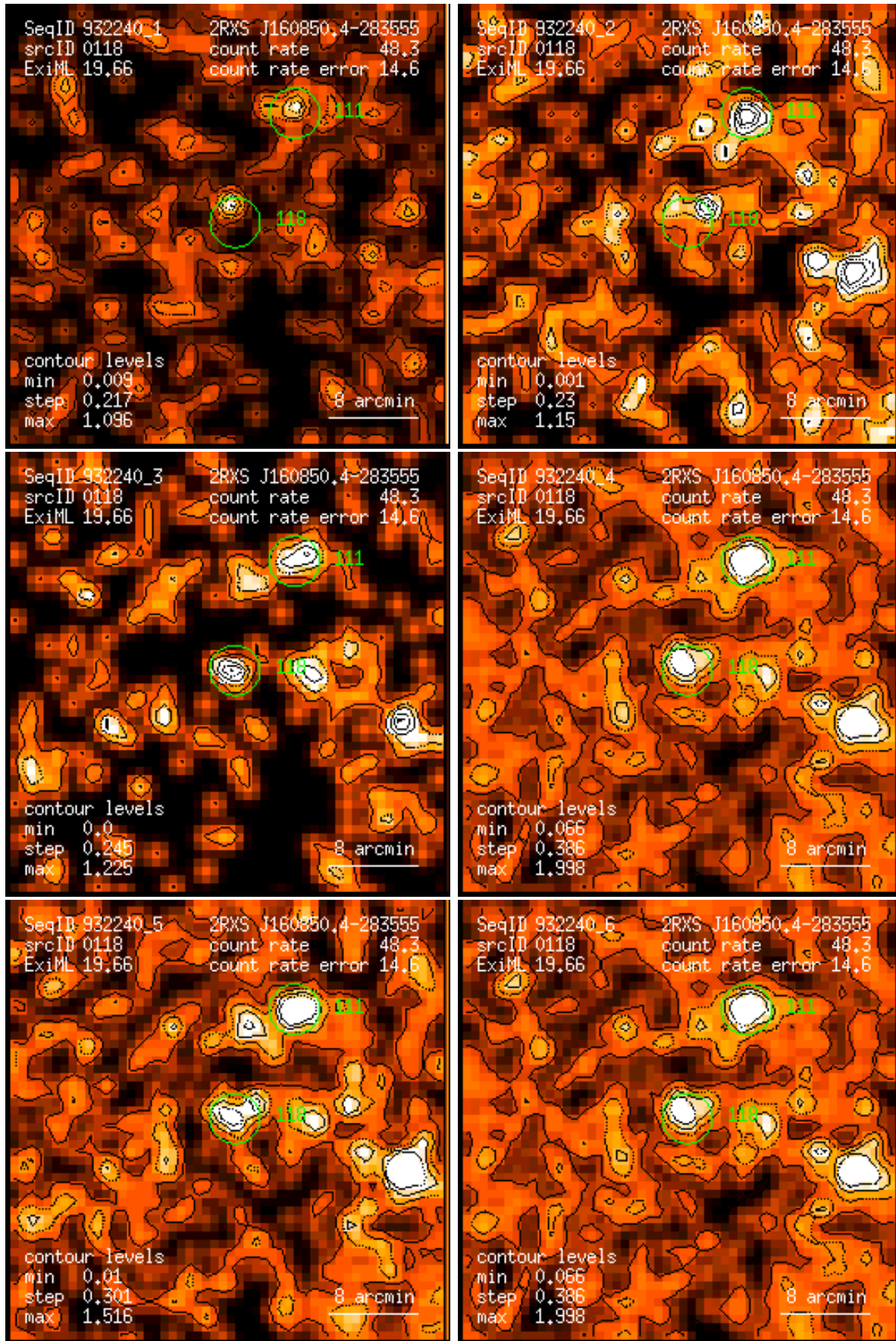
Figure 118: RASS 932240: detection 0118: band rate images, Gaussian filter: (1) PSPC channels 11 – 41, (2) 52 – 90, (3) 91 – 201, (4) 11 – 235, (5) 52 – 201, (6) 11 – 201. Broad band rates in counts/ks. Band rate contour levels in counts/ks/arcmin 2 .
