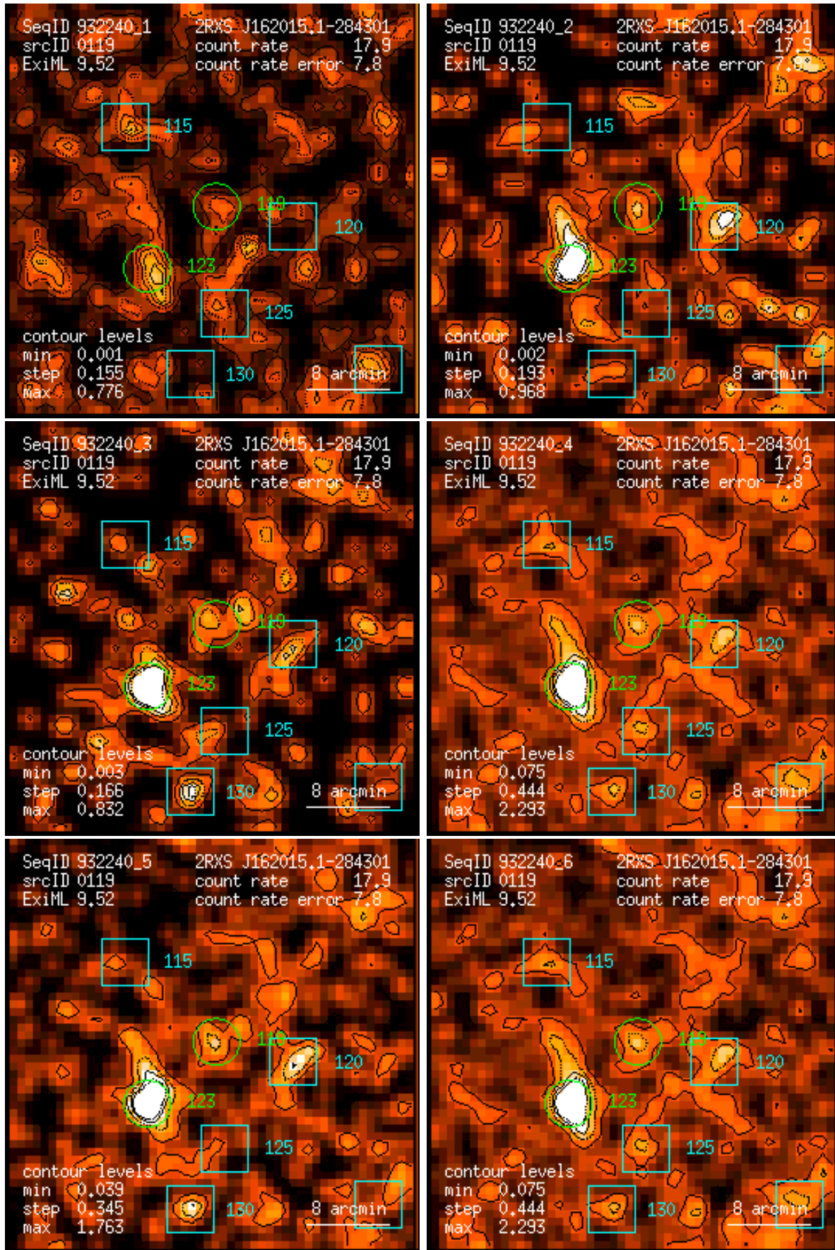
Figure 119: RASS 932240: detection 0119: band rate images, Gaussian filter: (1) PSPC channels 11 – 41, (2) 52 – 90, (3) 91 – 201, (4) 11 – 235, (5) 52 – 201, (6) 11 – 201. Broad band rates in counts/ks. Band rate contour levels in counts/ks/arcmin 2 .
