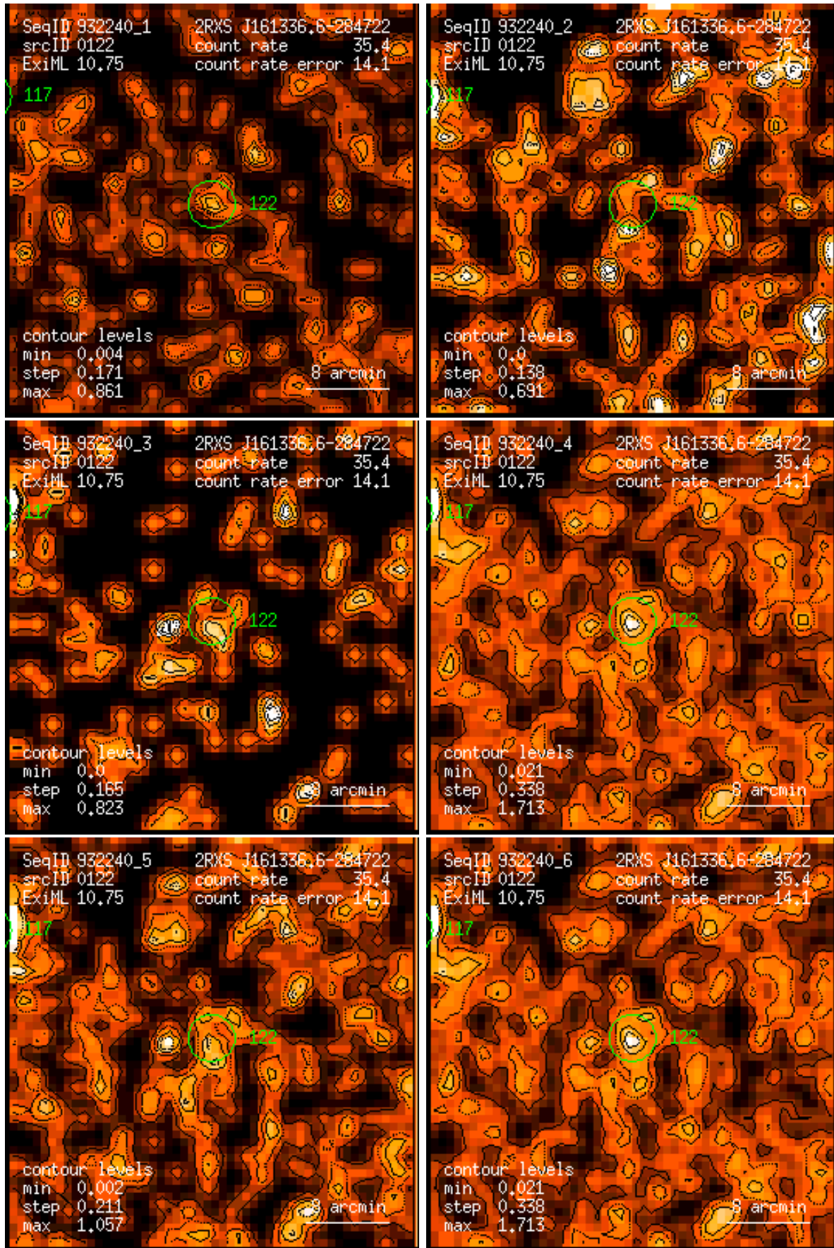
Figure 122: RASS 932240: detection 0122: band rate images, Gaussian filter: (1) PSPC channels 11 – 41, (2) 52 – 90, (3) 91 – 201, (4) 11 – 235, (5) 52 – 201, (6) 11 – 201. Broad band rates in counts/ks. Band rate contour levels in counts/ks/arcmin 2 .
