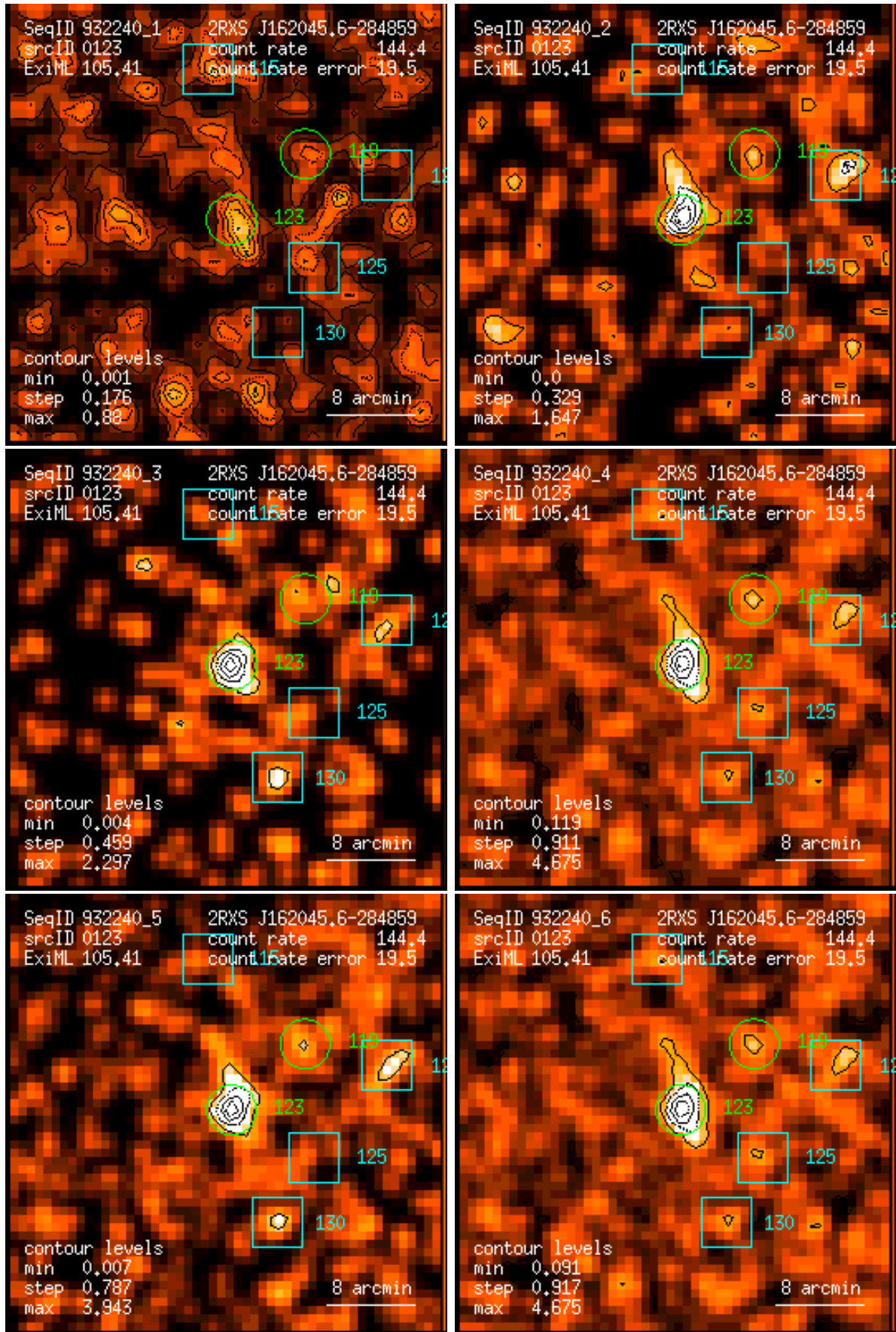
Figure 123: RASS 932240: detection 0123: band rate images, Gaussian filter: (1) PSPC channels 11 – 41, (2) 52 – 90, (3) 91 – 201, (4) 11 – 235, (5) 52 – 201, (6) 11 – 201. Broad band rates in counts/ks. Band rate contour levels in counts/ks/arcmin 2 .
